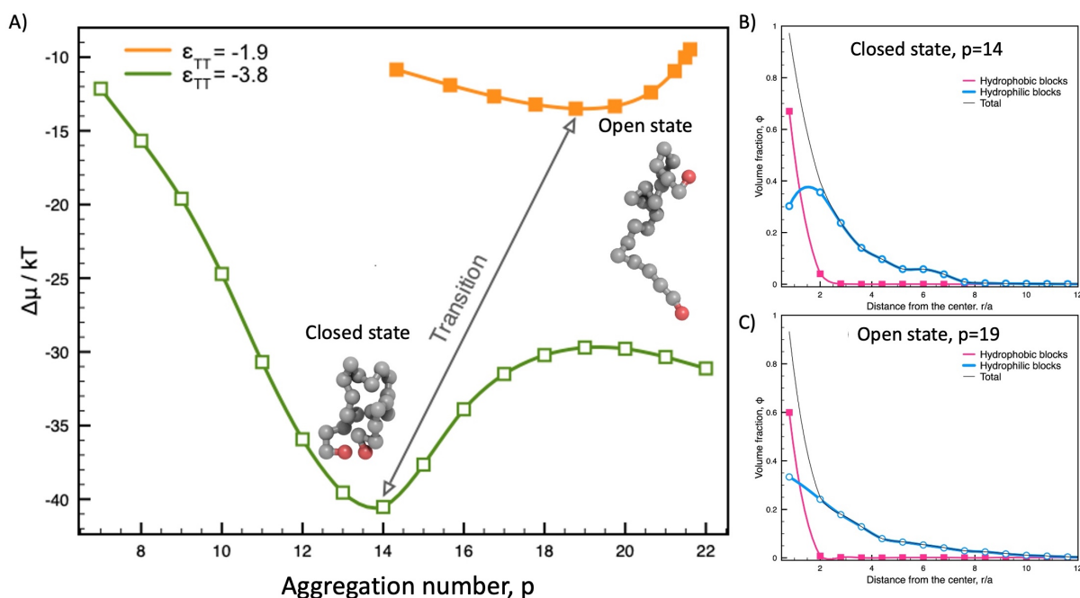
Figure 4: SCMF theory of telechelic micelles. A) Chemical potential difference \Delta\mu between monomers in the micelles and in the solution as a function of the aggregation number p for strong attraction, \varepsilon_{TT} = -3.8 , flower-like micelle, green curve, open squares, and weak attraction, \varepsilon_{TT} = -1.9 , star-like micelle, orange curve, closed squares. The corresponding to the minima volume fractions of hydrophobic blocks (red), hydrophilic blocks (blue) and the sum (grey) as a function of a distance from the center in the B) flower-like micelle, p = 14 and C) star-like micelle, p = 19 .
