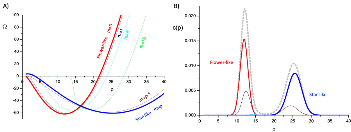
Figure 3: Aggregation of tri-block copolymers into micelles. A) Variation of \Omega with the aggregation number p and B) the corresponding size distributions for \gamma = 0.57 . The length of a hydrophilic block N = 500 and the length of the hydrophobic block L_c = 50 .
