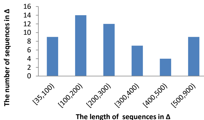
Figure 2: Distribution of the length of protein sequences in \Delta .
