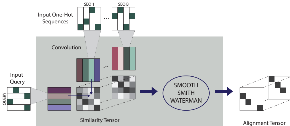
Figure 2: Learned alignment module (LAM). Residues are encoded as vectors through a convolution of the one-hot representations of the sequences. A similarity tensor is constructed by taking the dot product of the vectors for each sequence with the vectors for the query sequence. Smooth Smith-Waterman is applied, yielding smooth pairwise alignments between each sequence and the query sequence.
