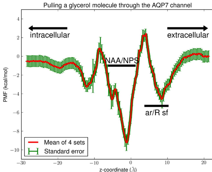
Fig. 6. PMF of glycerol throughout the AQP7 channel. The coordinates are set so that the center of membrane is located at z=0\text{\AA} . In the single-file region ( -11\text{\AA} < z < 9\text{\AA} ), the PMF is one dimensional. In the IC ( z < -11\text{\AA} ) or EC ( z > 9\text{\AA} ) side of the channel, the PMF is three dimensional. The three PMF wells (binding sites) are located at: Site 0, z \sim -1\text{\AA} ; Site 1, z \sim 9\text{\AA} ; Site 2, z \sim -11\text{\AA} .
