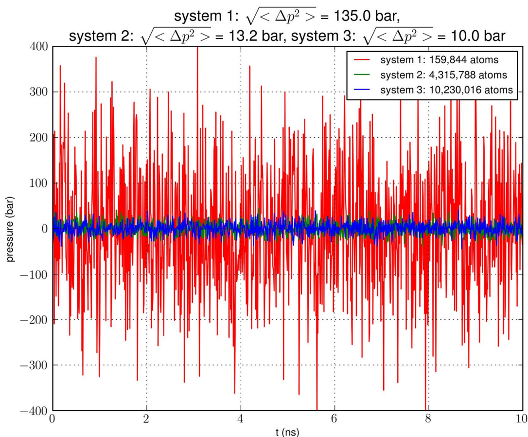
Fig 1. Pressure fluctuation in an NPT simulation of a small system (159,844 atoms) containing a single AQP7 tetramer, a large system (4,315,788 atoms) with 27 AQP7 tetramers, or a huge system (10,230,016 atoms) with 64 AQP7 tetramers. The pressure fluctuation is approximately proportional to the inverse of the system size in terms of atom numbers.
