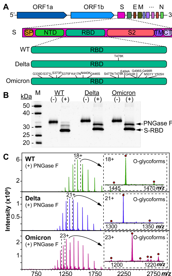
Figure 1. Protein mutational mapping and high-resolution top-down MS of S-RBD arising from the WT, Delta, and Omicron variants. (A) Architecture of SARS-CoV-2 genome and illustration of the protein sequence changes for the S-RBD variants. (B) SDS-PAGE of the S-RBD variants before (–) and after (+) PNGase F treatment. Gel lanes were equally loaded (300 ng), and gel staining was visualized by SYPRO Ruby. (C) Raw MS1 of intact S-RBD proteoforms collected on the 12 T FTICR-MS after PNGase F treatment for the WT, Delta, and Omicron variants. All identified O-glycoforms are annotated in the inset with a red circle.
