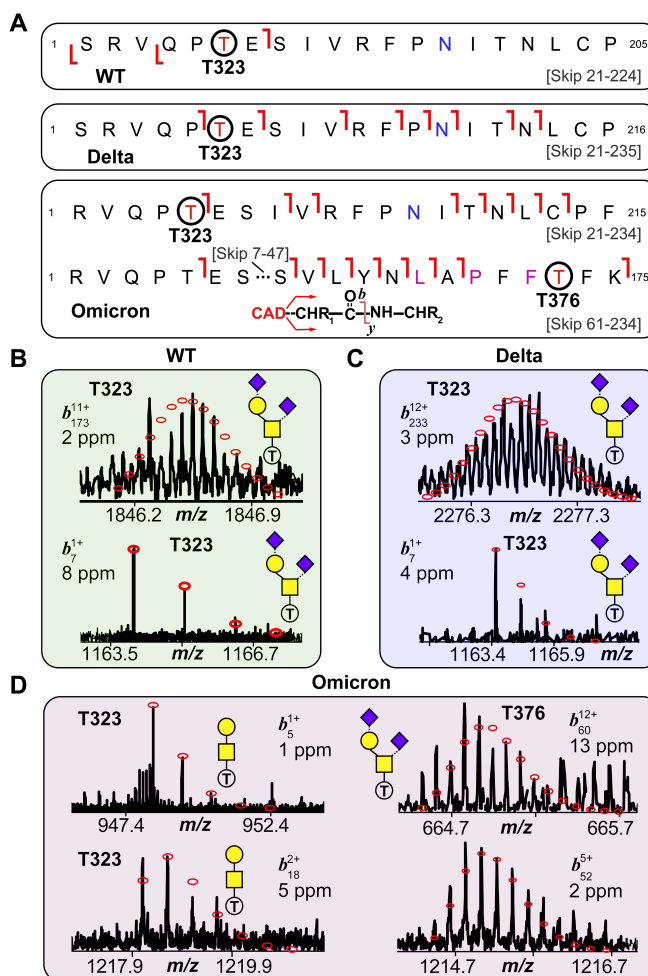
Figure 4. S-RBD O-glycosite localization by top-down TIMS-MS/MS. (A) Fragmentation mapping of the Core 1 type GalNAcGal(NeuAc) 2 glycan corresponding to the WT, Delta, and Omicron S-RBD variants. Amino acid sequence (Arg319-Phe541) was based on the entry name P0DTC2 (SPIKE_SARS2) obtained from the UniProtKB sequence database with appropriate amino acid substitutions made for the mutated Delta and Omicron variants. Cleavage of signal peptide tPA following cell expression results in the N-terminal Ser for the WT and Delta variants. The blue N (Asn) denotes deamidation following PNGase F treatment. Specific Omicron residue mutations are denoted with a pink residue. (B-D) Representative top-down MS/MS CAD fragment ions of intact WT ( b_{71}^{1+} and b_{17311}^{1+} ) (B), Delta ( b_{71}^{1+} and b_{22312}^{12+} ) (C), and Omicron ( b_{51}^{1+} , b_{182}^{2+} , b_{71}^{1+} , b_{17311}^{1+} ) (D) variants corresponding to the GalNAcGal(NeuAc) 2 O-glycoform shown in (A). WT and Delta variants showed complete O-glycosite occupation at Thr323. The Omicron variant was found to possess both Thr323 (left side; b_{51}^{1+} and b_{182}^{2+} ) and Thr376 (right side; b_{71}^{1+} and b_{17311}^{1+} ) as O-glycosites corresponding to the same Core 1 O-glycan structure. Theoretical isotopic distributions are indicated by the red dots and mass accuracy errors are listed for each fragment ion.
