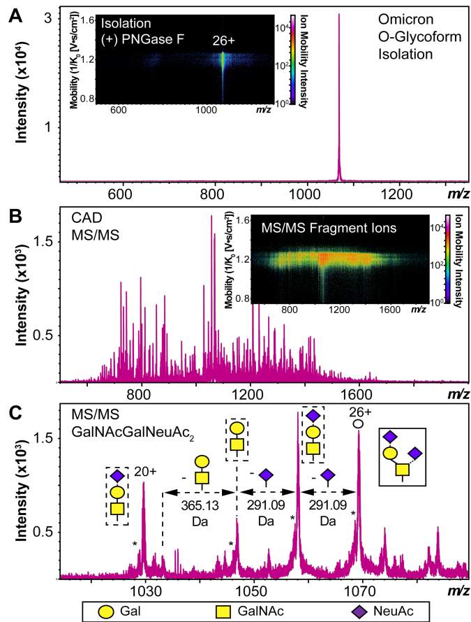
Figure 2. S-RBD O-glycoform analysis by TIMS-MS/MS. (A) Illustration of the isolation of a specific Omicron S-RBD glycoform ( z = 26+ , centered at 1069.4 m/z ) after PNGase F treatment using TIMS-MS. (Inset) Associated ion mobility heat map after isolation of the precursor. (B) Top-down MS/MS of Omicron S-RBD O-glycoform following CAD fragmentation of the isolated proteoform. A collision cell voltage of 22 eV was applied for this specific example. (C) Neutral loss O-glycan mapping of the Omicron S-RBD proteoform. Glycoform characterization reveals the specific S-RBD proteoform to have a Core 1 type GalNAcGalNeuAc 2 glycan structure. Assignments of the glycan structures are marked in the spectrum with the legend shown on the bottom. The hollow circle represents the 26+ charge state precursor ion corresponding to the 1069.4 m/z isolation. An asterisk “*” denotes an oxonium ion loss.
