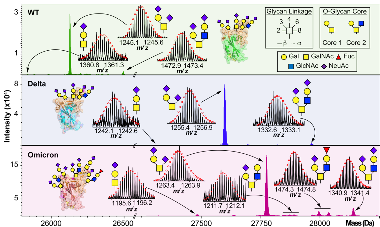
Figure 3. O-glycoform characterization of the S-RBD variants. Deconvoluted MS of the S-RBD proteoforms are shown with all major O-glycan assignments for the WT (green), Delta (blue), and Omicron (pink) variants. Insets show the isotopically and baseline resolved S-RBD proteoform MS spectra allowing for accurate determination of individual intact glycoforms. MS data were collected on the 12 T FTICR-MS. All individual ion assignments are within 1 ppm from the theoretical mass and theoretical isotopic distributions are indicated by the red dots. Assignments of the glycan structures are marked in the spectrum with the legend shown as an inset. PDB: 6M0J, 7WBQ, 7WBP.
