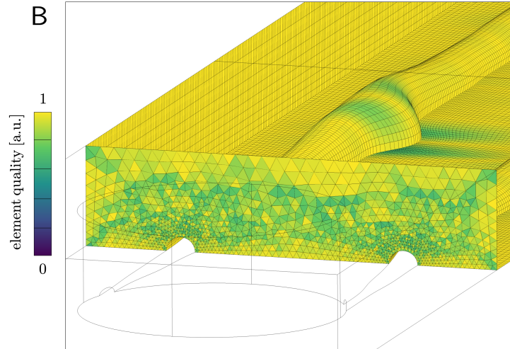
Fig. S4 (A) Element size map on the midplane. (B) Map of element quality on the source surface for the loft operation and on the surfaces of the swept domains
