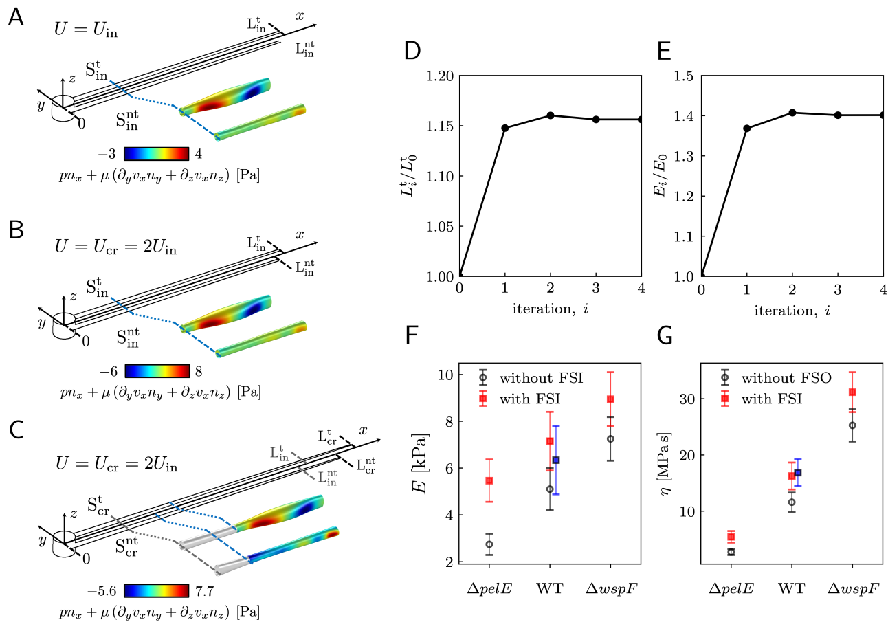
Fig. 5 (A) Schematic of the streamers during the initial stage of the creep-recovery test. The zoomed-in portion of streamers shows f_{in}(x) (Eq. (7)) in the region between x = 810 \mu m and x = 870 \mu m . f_{in}(x) is calculated with CFD using the initial shapes S_{in}^t and S_{in}^{nt} of the tracked and not tracked streamers, respectively, and U_{in} . (B) Schematic of the streamers during the creep stage of the test, when FSI is neglected. CFD simulations with the initial shapes S_{in}^t and S_{in}^{nt} and U_{cr} = 2U_{in} , gives f_{cr}(x) = 2f_{in}(x) , at low Re. (C) When taking FSI into account, f_{cr}(x_{cr}(x, t)) changes with time, because it depends on the time-dependent shape of the filaments S_{cr}^t(t) , S_{cr}^{nt}(t) (Eq. (12)). Our estimate of f_{cr}(x_{cr}(x, t^*)) with FSI was obtained by calculating the approximate shapes S_{cr}^t(t^*) , S_{cr}^{nt}(t^*) at time t = t^* \equiv 150 s , right after the elastic deformation. f_{cr}(x_{cr}(x, t^*)) is not trivially related to f_{in}(x) . We also see that the deformation is not the same on the two filaments, due to their different morphology. (D) Convergence plot for the elastically deformed length L and (E) E of the average PA14 WT streamer. (F, G) E and \eta calculated without FSI (open circles) and with the FSI correction calculated on the average streamer shapes (red squares). Blue squares for PA14 WT are obtained by calculating E and \eta with FSI for each experimental replicate and then by averaging the results.
