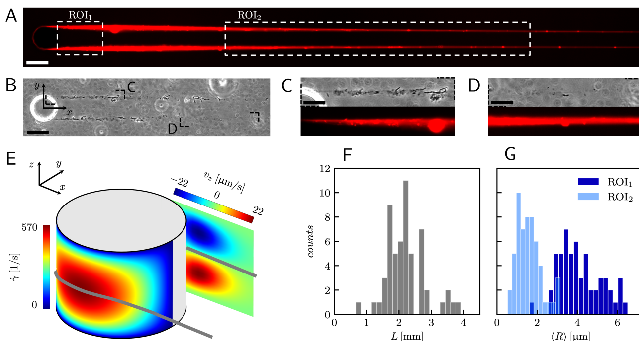
Fig. 1 (A) Representative fluorescence and (B) phase contrast images of PA14 biofilm streamers tethered to a micropillar. The images were acquired by focusing on the channel midplane. In (A) we show the regions of interest (ROI) where we calculated the average radius \langle R \rangle (ROI 1 and ROI 2 ) and where we acquired images during the rheological tests (ROI 2 ). ROI 1 goes 25 \mu\text{m} to 125 \mu\text{m} , while ROI 2 goes from 400 \mu\text{m} to 1665.6 \mu\text{m} . The reported image is composed of two adjacent fields of view stitched together. 33 Scale bars are 50 \mu\text{m} . (C, D) detailed view of the two regions marked in (B). Scale bars are 20 \mu\text{m} . (E) Schematic of the hydrodynamic features driving streamers formation. On one side of the pillar ( y < 0 ), we show the shear rate \dot{\gamma} at the surface. On the other side of the pillar ( y > 0 ), we show the z-component v_z of the velocity field on a vertical plane from x = 0 to x = 45 \mu\text{m} . The distributions reported here were numerically calculated in the absence of biofilm filaments and are symmetric with respect to the x - z plane. The grey lines mark the approximate position where biofilm streamers form. (F) Distributions of lengths and (G) radii (averaged over ROI 1 and ROI 2 ) of 15 h old biofilm streamers, formed in the microfluidic platform at a mean flow velocity of U = 2.1 \text{ mm/s} . The average length is \langle L \rangle = 2.22 \pm 0.08 \text{ mm} , while the average values of the radius are \langle R \rangle = 4.1 \pm 0.14 \mu\text{m} in ROI 1 and \langle R \rangle = 1.57 \pm 0.08 \mu\text{m} in ROI 2 . The uncertainties on the reported values are calculated as the standard deviation of the mean.
