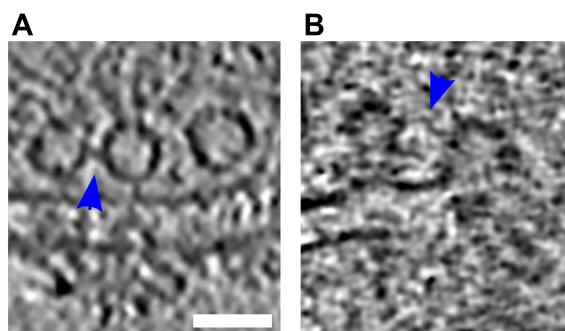
Figure S5: (A, B) Tomographic slices showing tethered connected vesicles. Blue arrows highlight the connectors. Scale bar, 50 nm.
