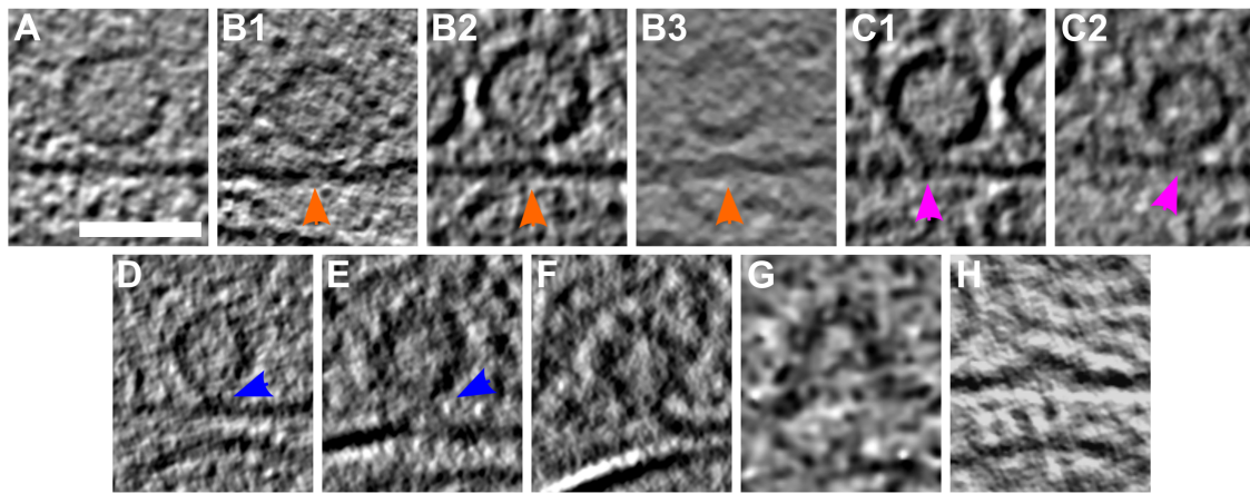
Figure 2: SV exocytosis morphology. Tomographic slice of non-stimulated (A) and stimulated rat synaptosomes (B-H). A) Image of a 2.2-nm thick tomographic slice showing a non-stimulated with SVs at the AZ and a straight PM. B1) Membrane curvature event, 2.2-nm thick tomographic slice. B2) Membrane curvature event, 6.5-nm thick tomographic slice. B3) Membrane curvature event, 2.24 nm thick tomographic slice. Orange arrows showing membrane curvature event. C1,C2) Lipid perturbations of PM and SV, 22-nm thick tomographic slices. The space between SV and PM is denser than in the non-stimulated synaptosomes (see pink arrow). D-F) Vesicles with a pore opening that might be on the way to full collapse fusion, 33-nm thick tomographic slice thickness: 22 nm (D), 30.8 (E), 33 nm (F). G) Wide pore opening, most likely on the way to full collapse fusion, 2.2-nm tomographic slice. H) Remaining bump at the end of full collapse fusion, 11-nm thick tomographic slice. Scale bar, 50 nm.
