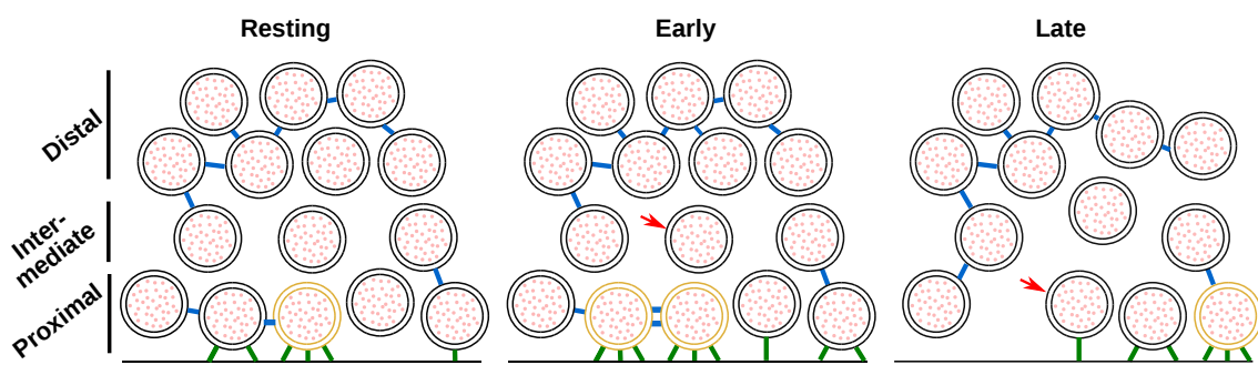
Figure 6: Model depicting a synapse transitioning from resting state to early and late fusion states. Tethering and connectivity changes upon synapse stimulation are depicted. Proximal non triple-tethered vesicles (black proximal SVs) gain additional tethers and some of them become triple-tethered (yellow SVs) shortly after stimulation. Primed vesicles then fuse with the plasma membrane (late fusion) and leave an empty space in the AZ cytoplasm. The number of connectors (depicted in blue) per proximal SV decreases in late fusion triple-tethered vesicles. The red arrow shows a vesicle initially located in the intermediate region, which diffuses to the proximal region in the late fusion state. Tethers are shown in green.
