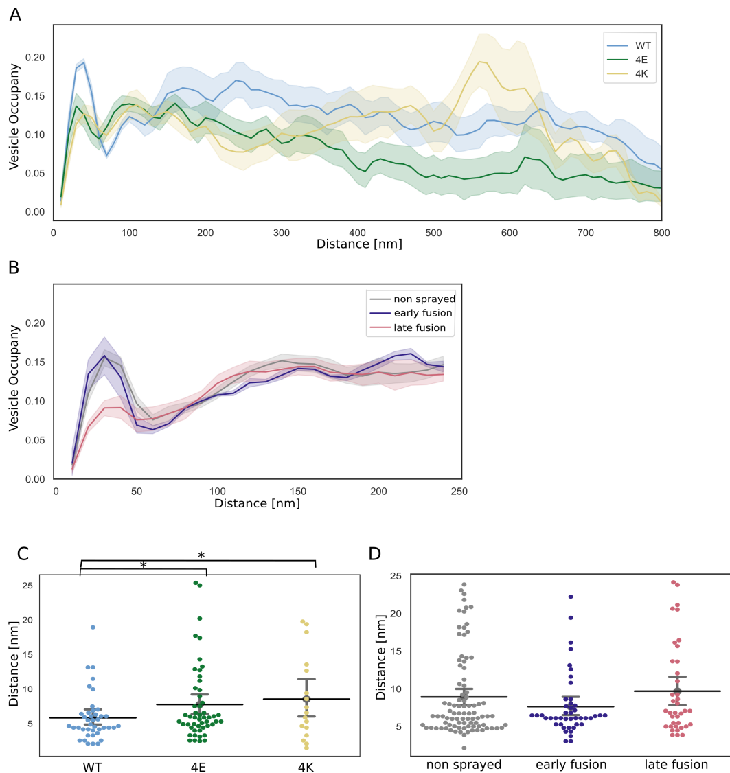
Figure 3: SV distribution. (A, B) Vesicle occupancy expressed as fraction of cytosol volume occupied by vesicles as a function of distance to AZ in (A) cultured neurons and (B) synaptosomes. Each solid line represents the mean occupancy value for the experimental group, while the shaded areas depict twice the standard error of the mean (SEM). (C, D) Distance of proximal SVs from the AZ. Horizontal line: mean; whiskers: 2xSEM interval. Statistical test: multiple all against control pairwise ANOVA comparisons with Benjamini-Hochberg correction; * : P < 0.05
