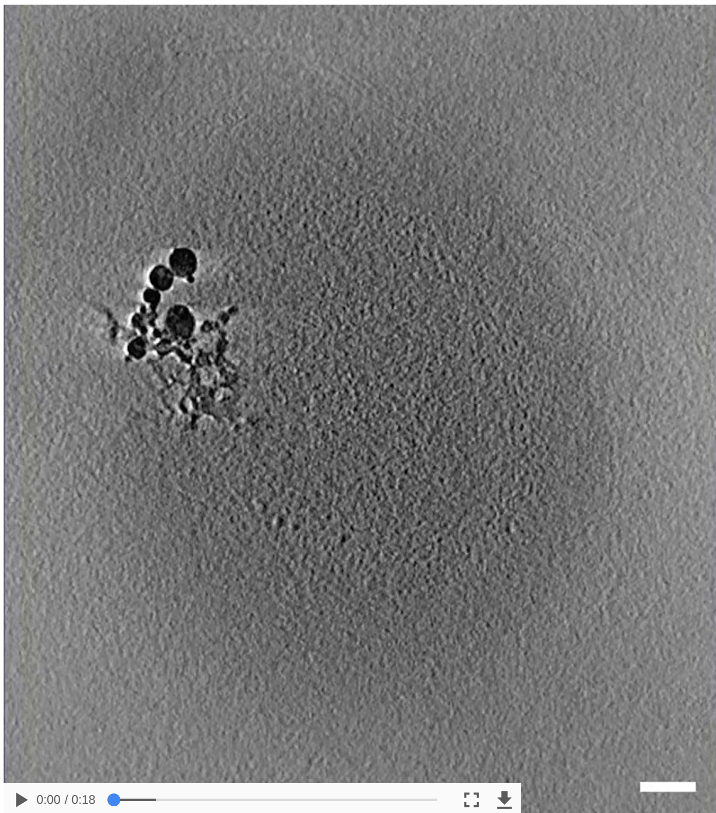
Movie S1: Tomogram with segmentation of synaptosome with late fusion events. off-white = cell outline; pink = active zone; blue = synaptic vesicles; dark green = mitochondria; light green = large vesicles; yellow = connectors, red = tethers, scale bar 100nm
