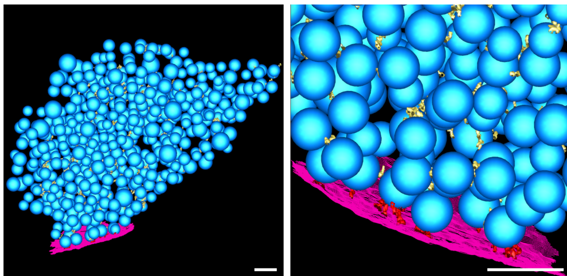
Figure S3: Segmented tomogram of a SNAP-25 4E neuron. (left) Overview. (right) Detail. Blue: synaptic vesicles; purple: active zone plasma membrane; yellow: connectors; red: tethers. Scale bar: 100 nm.
