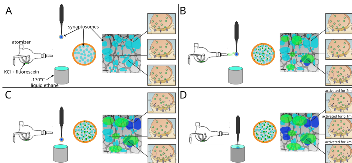
Figure S1: Schematic representation of a spray-mixing plunge-freezing experiment. In a single experiment different synaptosomes get stimulated for between less than 1 ms and 7 ms. An EM-grid is held by tweezers and is covered with synaptosomes in HBM-solution. A magnified view of a grid squares shows synaptosomes in blue and their synaptic state of three synaptosomes is represented on the rightmost part of each panel. Panel (A) represents the situation right after blotting off solution excess. The grid is accelerated towards the spray and the cryogen. Panel (B) shows a snapshot of the experiment when the grid crosses the spray, 7 ms before the freezing. Some fluorescently dyed droplets containing HBM with 52 mM KCl land on the grid and are depicted in green. At this time point, a synaptosome located at the impact point of a droplet is activated and is depicted in dark blue. Panel (C) shows a snapshot 5 ms later, i.e. 2 ms before freezing. As KCl diffuses away from droplet impacts points, another synaptosomes gets activated because, locally KCl concentration has reached a concentration to depolarize enough the synaptosome so that voltage-gated calcium channels open. Panel (D) shows a synaptosome at the time of impact with ethane. 0.1 ms before freezing a third synaptosome got exposed to a high enough concentration of KCl and got stimulated.
