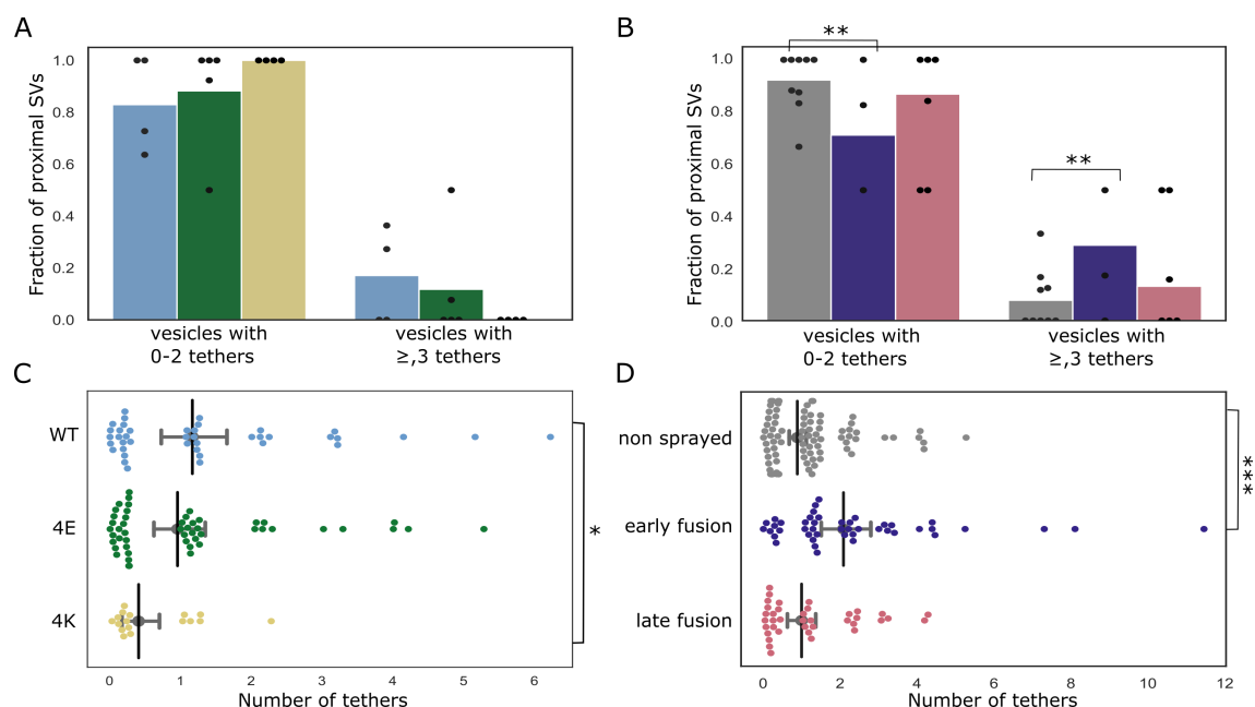
Figure 4: Proximal SV tethering. (A, B) Fraction of proximal SVs that are triple tethered. Each bar shows the overall fraction of all proximal SVs from a given experimental condition. Each dot represents the value of an individual synapse. Statistical test: multiple all against control pairwise \chi^2 -test with Benjamini-Hochberg correction. (C, D) Number of tethers per proximal SV. Each dot represents an individual SV. The vertical line represents the mean value, and the horizontal whiskers correspond to the 95% confidence interval. Statistical test: multiple all against control pairwise ANOVA comparisons with Benjamini-Hochberg correction; *: P < 0.05 , **: P < 0.01 , ***: P < 0.001 .
