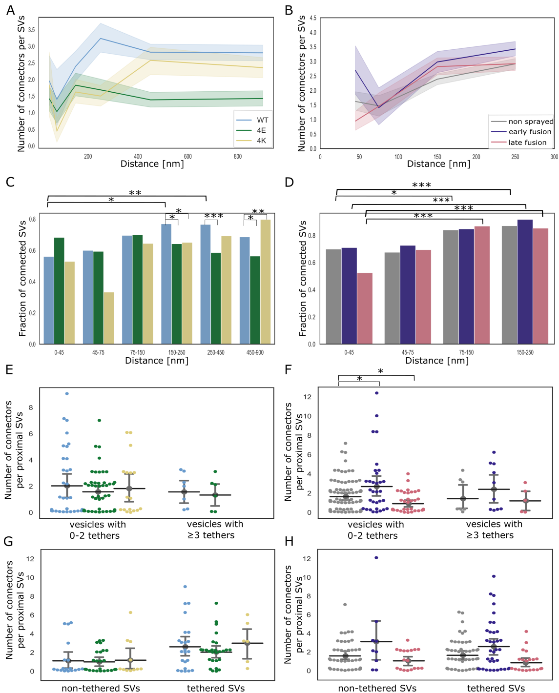
Figure 5: SV connectivity. (A, B) Number of connectors per SV as a function of their distance to the AZ PM for mouse neurons (A) and rat synaptosomes (B). Each solid line represents the average value of all SVs belonging to a particular experimental condition. Shaded areas represent 2xSEM interval ranges. Statistical tests: multiple all against reference pairwise ANOVA comparisons with Benjamini-Hochberg correction. Within a single experimental condition, the reference was the proximal distance group; within a single experimental group, the reference was the WT genotype or non-sprayed synaptosomes. (C, D) Fraction of connected vesicles as a function of distance to the AZ PM for mouse neurons (C) and rat synaptosomes (D). Statistical test: multiple all against reference pairwise \chi^2 -test with Benjamini-Hochberg correction; references were defined as in (A) and (B). (E, F) Number of connectors per proximal SV belonging or not to the RRP for mouse neurons (E) and rat synaptosomes (F). (G, H) Number of connectors per tethered or non-tethered proximal SV for mouse neurons (G) and rat synaptosomes (H). Statistical tests in (E-H): multiple all against control pairwise ANOVA comparisons with Benjamini-Hochberg correction. Control was WT genotype or non-sprayed synaptosomes. In all statistical tests, *: P < 0.05 , **: P < 0.01 , ***: P < 0.001 .
