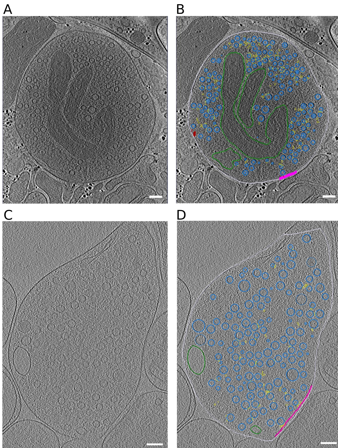
Figure S2: Representative slices through tomograms. (A, B) Tomographic slice without (A) and with (B) segmentation of synaptosome with late fusion events. (C, D) Tomographic slice without (C) and with (D) segmentation of WT SNAP-25 neurons. Segmentation colors: off-white = cell outline; pink = active zone; blue = synaptic vesicles; green = mitochondria; yellow = connectors, red = tethers. Scale bar, 100 nm.
