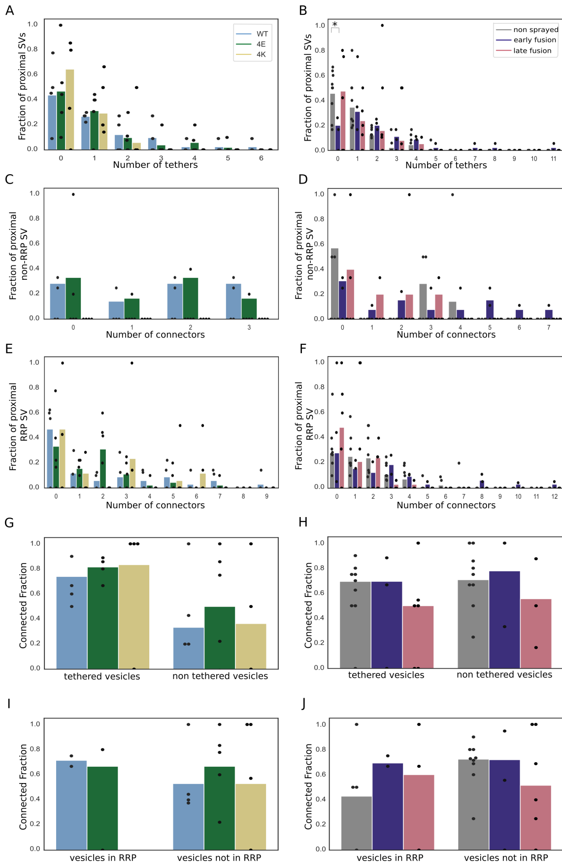
Figure S4: (A, B) Histogram of the number of tethers per proximal SV. Statistical test: pairwise \chi^2 -test between control and each experimental condition in the 0-tether group with Benjamini-Hochberg correction. *: P < 0.05 . (C, D) Histogram of the number of connectors per proximal non-RRP SV. (E, F) Histogram of the number of connectors per RRP SV. (G, H) Histogram of connected SV amongst tethered or non-tethered proximal SVs. (I, J) Histogram of connected SV amongst proximal non-RRP or RRP SVs. (A, C, E, G, I) Synapses in mouse cultured neurons. (B, D, F, H, J) Rat synaptosomes.
