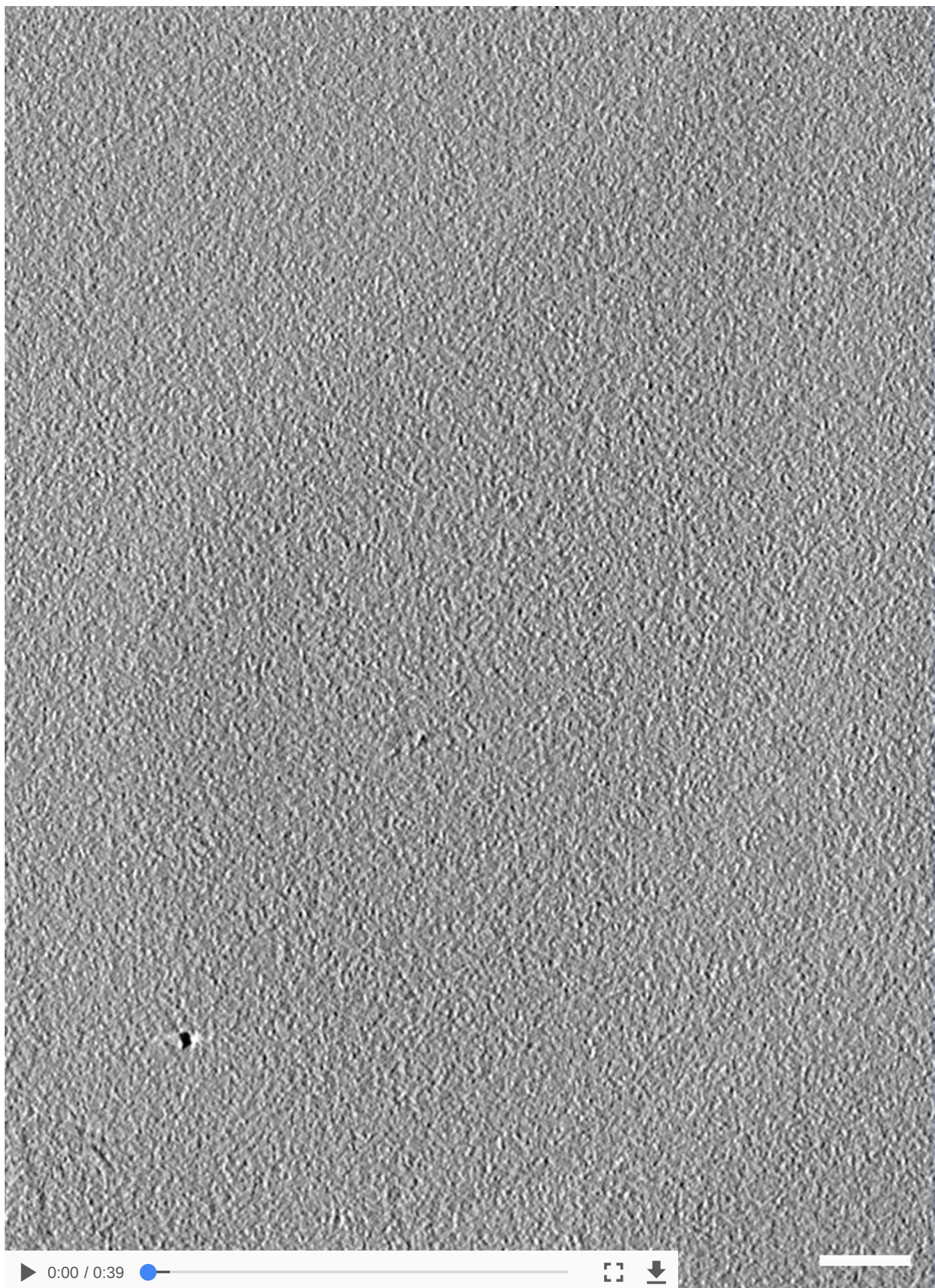
Movie S2: Tomogram with segmentation of WT SNAP-25 neurons. off-white= cell outline; pink = active zone; blue = synaptic vesicles; green = large vesicles; yellow = connectors, red = tethers, scale bar 100nm
