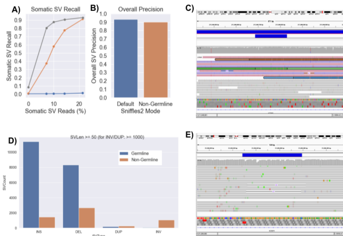
Figure 4: Recovery of somatic SVs using the Sniffles2 non-germline mode A+B) benchmark of mixtures of HG002 with HG004. We spiked HG002 in various concentrations and measured the recall (A) and precision (B) of Sniffles2 at different variant allele frequencies. C) Example of a false positive inversion (small blue bar on top) caused by likely chimeric reads. The three supporting INV reads are highlighted in brown, green, blue. Other likely chimeric reads are shown in light blue and red. D) Overview of SV types identified as germline (blue) and non-germline events in the MSA patient brain sample. E) Example of mosaic repeat contraction detected by Sniffles2.
