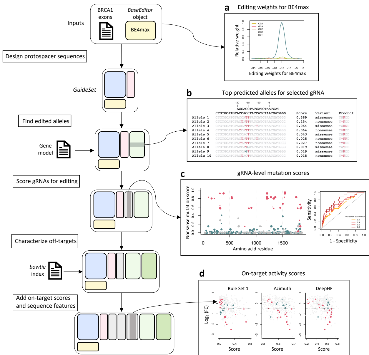
Figure 3. crisprDesign workflow to design gRNAs tiling BRCA1 using the base editor BE4max.
