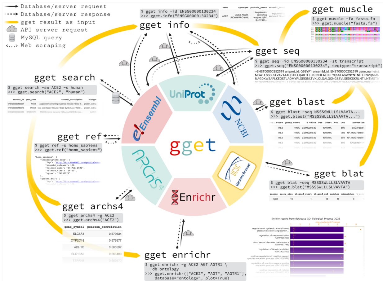
Figure 1 Overview of the nine gget tools and the public databases they access. One simple command line ($) example and its Python (>>>) equivalent are shown for each tool with the corresponding output.
