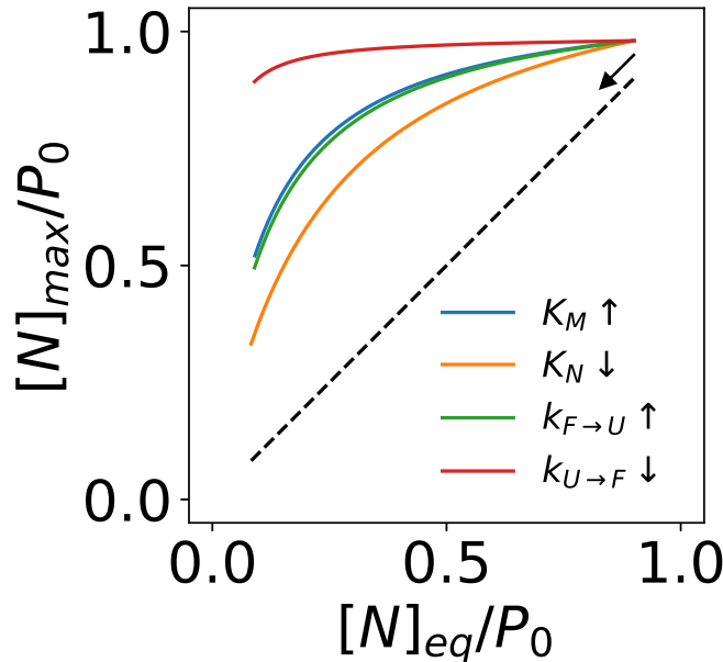
FIG. 5: The capacity of ATP-driven chaperones to maintain elevated native fractions in response to destabilizing mutations in a protein substrate. The kinetic parameters of the wild-type protein are K_M = 10^2 , K_F = 10 , K_N = 10^2 , k_{U \rightarrow F} = 0.1s^{-1} , and k_a = 10^6 M^{-1} \cdot s^{-1} ; the concentration of the open chaperone is set to [O] = 1\mu M .
