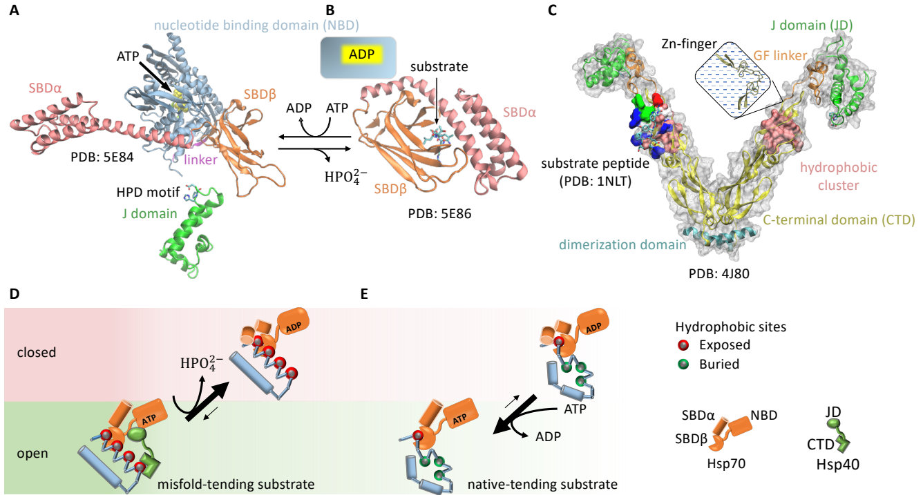
FIG. 3: Cochaperone Hsp40 enables Hsp70 to change the balance between its open and closed states in response to the conformation of a bound substrate. A . The ATP-bound, open state of Hsp70, which allows rapid binding and unbinding of the substrate. B . The ADP-bound, closed state of Hsp70, with slow binding and unbinding of the substrate. SBD: substrate binding domain. C . The structure of the Hsp40 cochaperone, including CTD that can bind to exposed hydrophobic sites on a substrate and the J domain that can stimulate the ATP hydrolysis of Hsp70. D . An Hsp70 bound to a misfold-tending substrate molecule with many exposed hydrophobic sites is likely to be in proximity to an Hsp40 bound to the same substrate molecule, thus the Hsp70 will be stimulated in ATP hydrolysis, which drives the Hsp70 to its ADP-bound, closed state. E . An Hsp70 bound to a native-tending substrate molecule with few exposed hydrophobic sites is unlikely to have a nearby Hsp40 and thus unlikely to be stimulated in ATP hydrolysis, and nucleotide exchange drives the Hsp70 toward its ATP-bound, open state.
