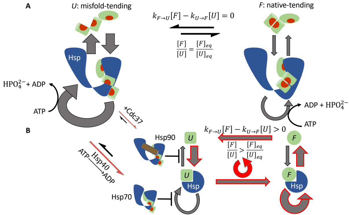
FIG. 4: Reactive flux in chaperone-mediated non-equilibrium protein folding. A. Under the symmetry conditions, there are two independent ATP-driven chaperone cycles: one with a higher reactive flux for a substrate in the misfold-tending ( U ) conformation (left) and one with a lower reactive flux for a substrate in the native-tending ( F ) conformation (right). There is no net flux between the substrate's two conformations, and the ratio [F]/[U] is the same as its chaperone-free equilibrium value. B. Cochaperones break the kinetic symmetry. The release of a substrate in the U conformation from the chaperone is inhibited: Cdc37 assists Hsp90 to retain the substrate and Hsp40 stimulates ATP hydrolysis and closure of Hsp70. This restricts the reactive flux to release a substrate in the U conformation, forcing a partial diversion of the flux to the conformation conversion from U \cdot \text{Hsp} to F \cdot \text{Hsp} and resulting in a net reactive flux of U \rightarrow U \cdot \text{Hsp} \rightarrow F \cdot \text{Hsp} \rightarrow F \rightarrow U (red cycle), which elevates the ratio [F]/[U] above its chaperone-free equilibrium value.
