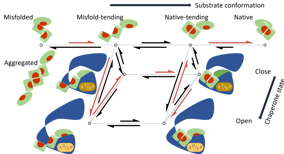
FIG. 1: A mechanistic model of chaperone-mediated non-equilibrium protein folding that couples the state cycle of the chaperone and the conformational dynamics of its substrate. The chaperone undergoes a cycle of open and closed conformations, driven by ATP hydrolysis and nucleotide exchange. The protein substrate can transition among four classes of conformations: Misfolded ( M ), Misfold-tending ( U ), Native-tending ( F ), and Native ( N ). The lengths of the reaction arrows signify the corresponding reaction rates. The red arrows indicate the predominant folding pathway.
