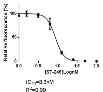
Figure S1: ST-246 inhibits VACV ANCHOR TM -GFP propagation at nM concentration. A) Reconstruction of 12 imaging fields captured on a CX7 CellInsight HCS microscope 48h post infection with indicated concentration of ST-246. Blue: nuclei, green VACV ANCHOR TM B/C) Quantification of the impact of ST-246 on the number of infected cells at 48 h (B) and 72 h(C) post-infection. IC 50 and R 2 are indicated.
