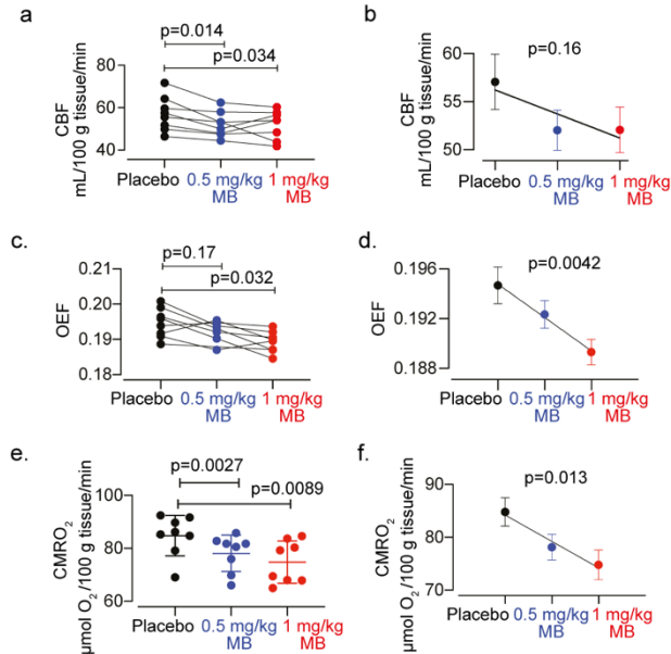
Figure 2: Effect of MB on CBF, OEF and CMRO 2 in healthy human subjects (n=8).
