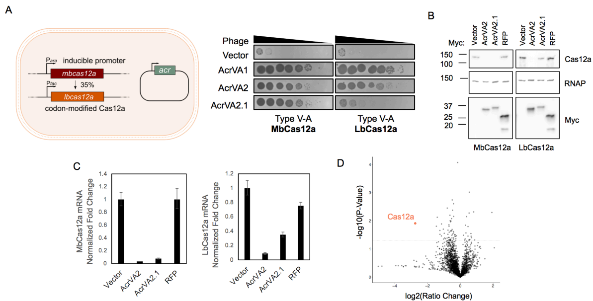
Figure 1. AcrVA2 specifically downregulates mRNA and protein of divergent Cas12a orthologs. (A) Left: Schematic of Pseudomonas aeruginosa strains engineered to express MbCas12a or codon-modified LbCas12a from inducible promoters and acr genes from plasmids. Right: Phage plaque assay with ten-fold serial dilutions of phage to assess CRISPR-Cas12a inhibition. (B) Western blot on bacterial lysates expressing myc-tagged anti-CRISPR or control proteins and Cas12a. RNAP, RNA polymerase (loading control). (C) qRT-PCR on mRNA from bacterial lysates expressing Cas12a and anti-CRISPR protein or control. Error bars indicate standard deviation. (D) Volcano plot for transcriptomic analysis. mRNA was extracted from bacteria expressing MbCas12a and AcrVA2 or controls. \log_2(\text{Ratio Change}) is the mean expression level for samples expressing AcrVA2 or AcrVA2.1 relative to controls (see methods for details). Each dot represents one gene. Dotted line indicates p-value of 0.05.
