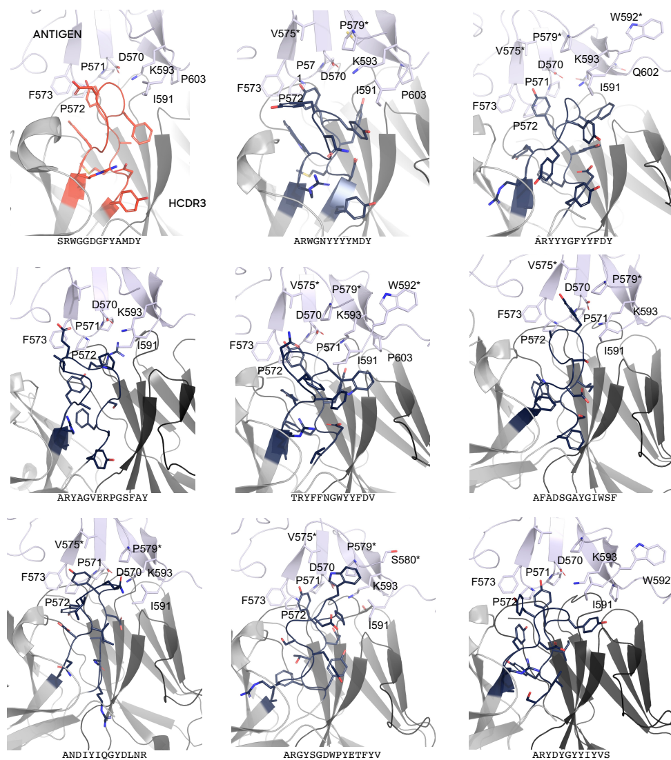
Fig S7. Stick representations of HCDR3-epitope interfaces. Residues were selected using a 5Å cutoff between HCDR3 and epitope residues (computed over all atoms). The trastuzumab HCDR3 loop is colored red (top left) and the de novo HCDR3 loops are colored blue. Epitope residues are labeled according to crystal structure PDB:1N8Z. An * denotes novel epitope residues in the de novo HCDR3 complexes that are not observed in the trastuzumab-HER2 complex.
