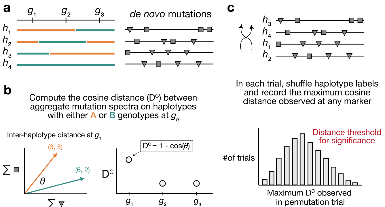
Figure 1: Overview of inter-haplotype distance method for discovering mutator alleles. a) A population of four haplotypes has been genotyped at three informative markers ( g_1 through g_3 ); each haplotype also harbors unique de novo germline mutations. In practice, de novo mutations are partitioned by k -mer context; for simplicity in this toy example, de novo mutations are simply classified into two possible mutation types (grey squares represent C>(A/T/G) mutations, while grey triangles represent A>(C/T/G) mutations). b) At each informative marker g_n , we calculate the total number of each mutation type observed on haplotypes that carry either parental allele (i.e., the aggregate mutation spectrum) using all genome-wide de novo mutations. For example, haplotypes with A (orange) genotypes at g_1 carry a total of three "triangle" mutations and five "square" mutations, and haplotypes with B (green) genotypes carry a total of six triangle and two square mutations. We then calculate the cosine distance between the two aggregate mutation
