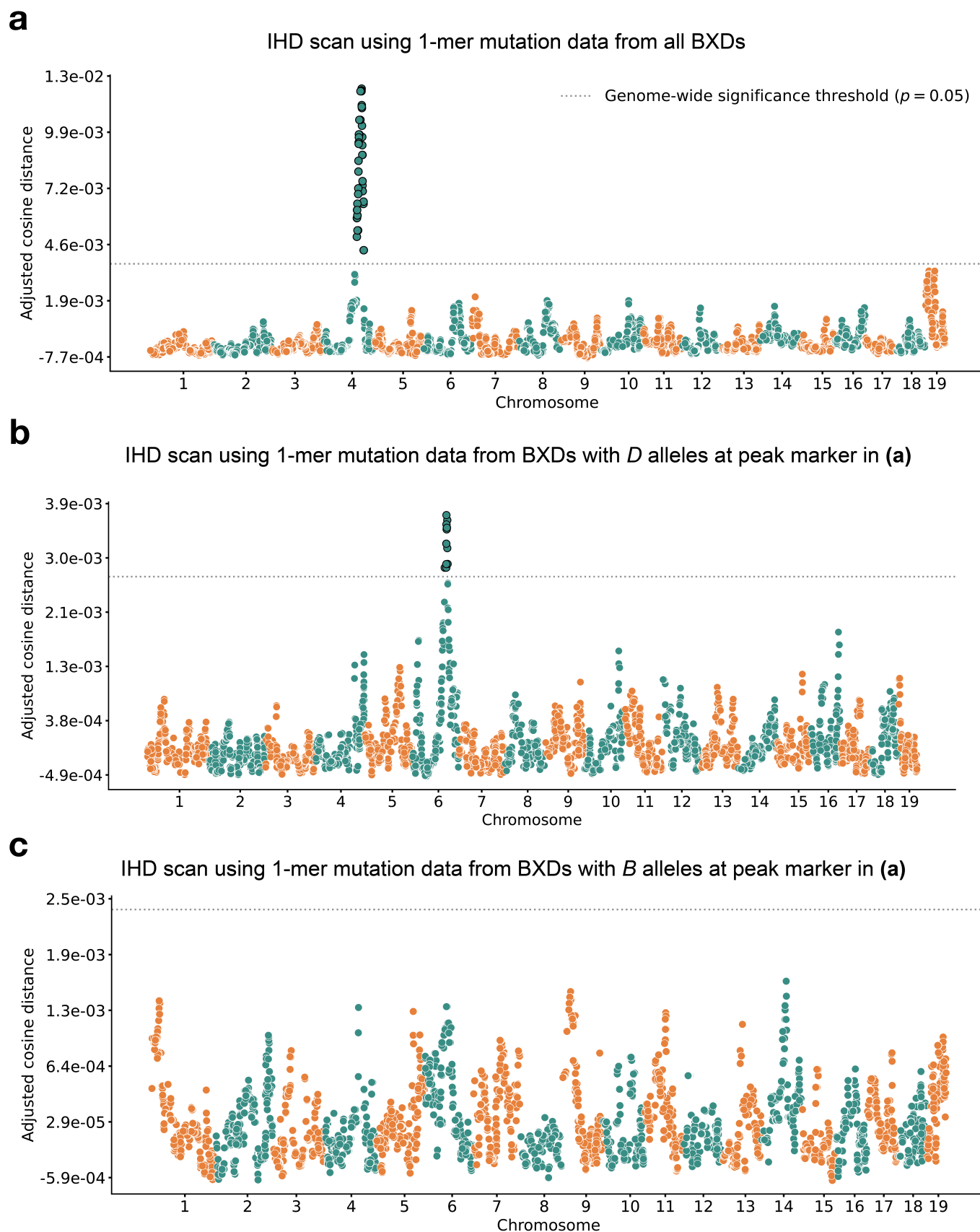
Figure 2: Results of inter-haplotype distance scans in the BXDs. a) Adjusted cosine distances between aggregate 1-mer de novo mutation spectra on BXD haplotypes ( n = 117 haplotypes; 65,552 total mutations) with either D or B alleles at 7,321 informative markers. Cosine distance threshold at p = 0.05 was calculated by performing 10,000 permutations of the BXD mutation data, and is shown as a dotted grey line. b) Adjusted cosine distances between aggregate 1-mer de novo mutation spectra on BXD haplotypes with D alleles at rs27509845 ( n = 66 haplotypes; 42,171 total mutations) and either D or B alleles at 7,276 informative markers. Cosine distance threshold at p = 0.05 was calculated by performing 10,000 permutations of the BXD mutation data, and is shown as a dotted grey line. c) Adjusted cosine distances between aggregate 1-mer de novo mutation spectra on BXD haplotypes with B alleles at rs27509845 ( n = 44
