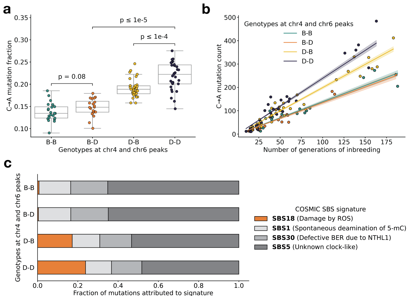
Figure 3: BXD mutation spectra are affected by alleles at both mutator loci. a) C>A de novo germline mutation fractions in BXDs with either D or B genotypes at markers rs27509845 (chr4 peak) and rs46276051 (chr6 peak). Distributions of C>A mutation fractions were compared with two-sided Mann-Whitney U-tests; annotated p-values are uncorrected. B-B vs. B-D comparison: U-statistic = 149.0, p = 7.58e-2 ; B-D vs D-D comparison: U-statistic = 21.0, p = 2.61e-8 ; D-B vs D-D comparison: U-statistic = 232.5, p = 6.99e-5 . b) The count of C>A de novo germline mutations in each BXD was plotted against the number of generations for which it was inbred. Lines represent predicted C>A counts in each haplotype group from a generalized linear model (Poisson family, identity link), and shading around each line represents the 95% confidence interval. c) Germline mutations in each BXD were assigned to COSMIC SBS mutation signatures using SigProfilerExtractor [27]. After grouping BXDs by their genotypes at rs27509845 and rs46276051, we calculated the fraction of mutations in each group that was attributed to each signature. The proposed etiologies of each mutation signature are: SBS1 (spontaneous deamination of methylated cytosine nucleotides at CpG contexts), SBS5 (unknown, clock-like signature), SBS18 (damage by reactive oxygen species, related to SBS36 and defective base-excision repair due to loss-of-function mutations in MUTYH), and SBS30 (defective base-excision repair due to NTHL1 mutations).
