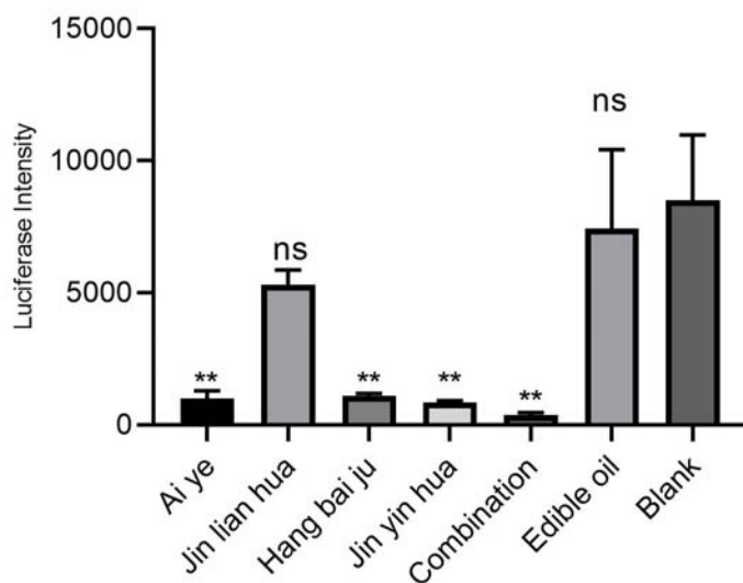
Fig 4 Combination of volatile oil inhibits SARS-CoV-2 pseudoviral infectivity in vitro.
