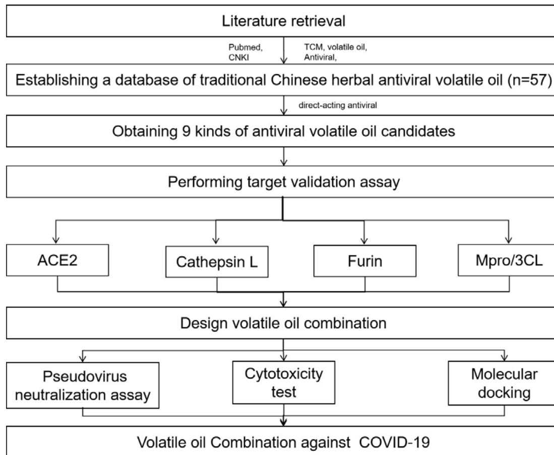
Fig 1. Workflow of this study.
