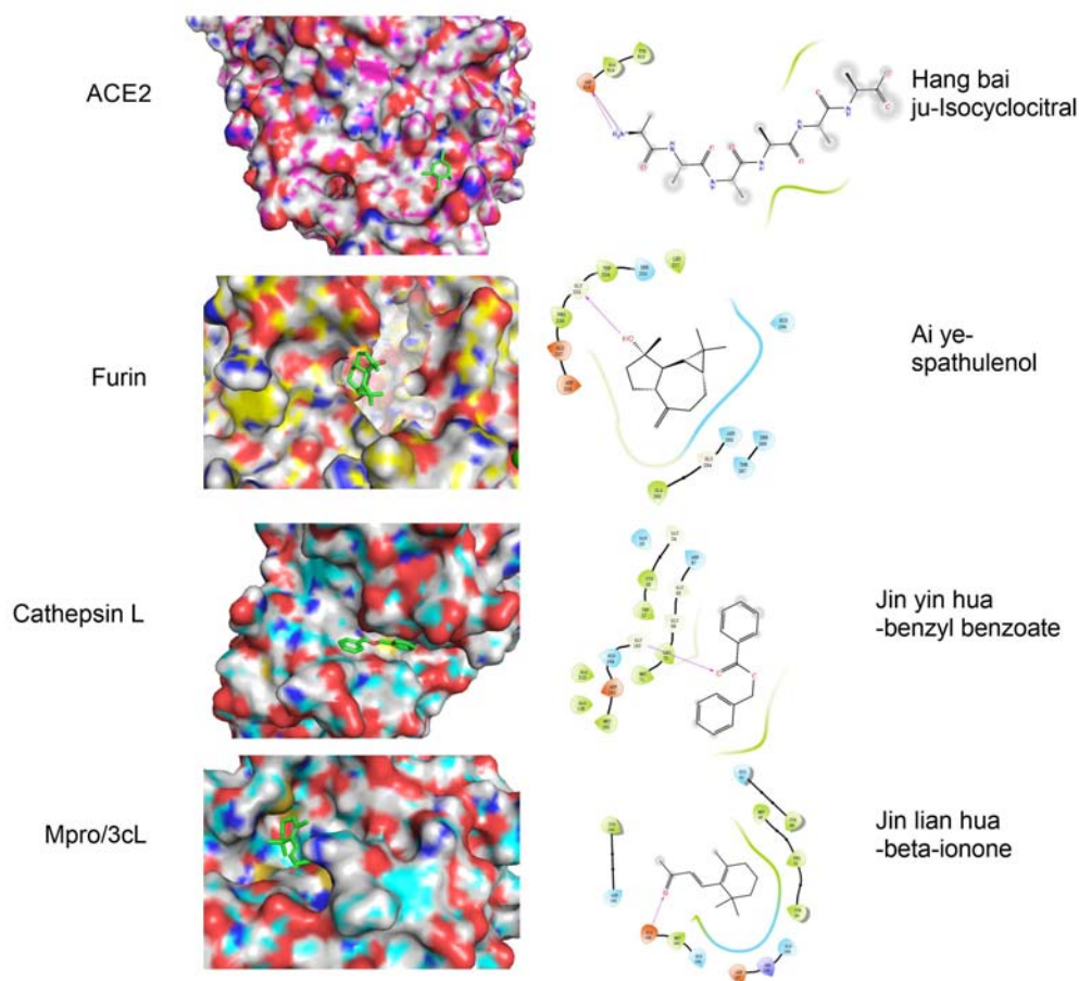
Fig 6 Molecular docking of representative components of Jin yin hua, Jin lian hua, Ai ye and Hang bai ju with Cathepsin L, Mpro/3cL, Furin and ACE2 Proteins, respectively
