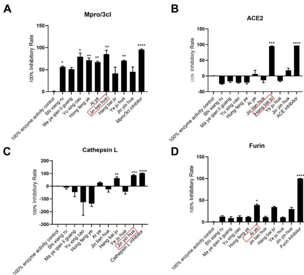
Fig 3. Target screening of volatile oil against SARS-CoV-2. (A) Jin lian hua inhibited the activity of Mpro/3cl at maximal levels. (B) Hang bai ju inhibited the activity of ACE2 at maximal levels(C) Jin yin hua inhibited the activity of Cathepsin L at maximal levels. (D) Ai ye inhibited the activity of Furin at maximal levels. The data represent results combined from three independent experiments. * p < 0.05 , ** p < 0.01 , *** p < 0.001 compared to 100% enzyme activity control.
