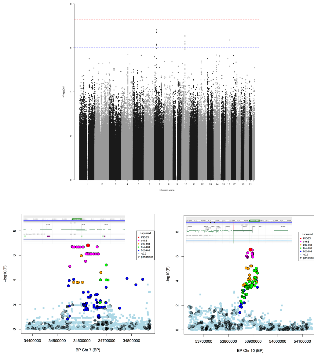
Figure 1: Results of GWAS Analysis for Chlamydia trachomatis seropositivity using EMMAX (A) Manhattan plot showing index SNPs with P_{EMMAX} < 1 \times 10^{-6} . There were two regions of within-gene SNP association with Chlamydia trachomatis serological response. (B) The Chr 7 : 34560375 - 34666861 region, within the non-protein coding NPSR1 Antisense RNA 1 ( NPSR1-ASI ) and immediately upstream of the G protein coupled receptor coding Neuropeptide S Receptor 1 ( NPSR1 ). (C) The Chr 10 : 53873323-56733116 region, within the gene encoding Protein Kinase, CGMP-Dependent, Type I ( PRKGI ), a mediator of the nitric oxide/cGMP signaling pathway, which has roles in immune function and GPCR signalling.
