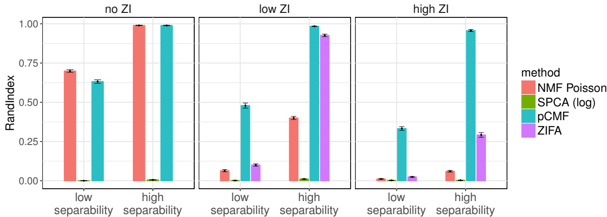
Figure 1: Adjusted Rand Index comparing clusters found by a \kappa -means algorithm (applied to \hat{U} with \kappa = 3 ) and the original groups of individuals, for different levels of zero-inflation and different levels of separation between groups of individuals in the data. The number of components is set to K = 3 . Data are generated with n = 100 , p = 1000 , 3 groups of individuals and 70% of noisy variables. Average values and deviation are estimated across 100 repetitions.
