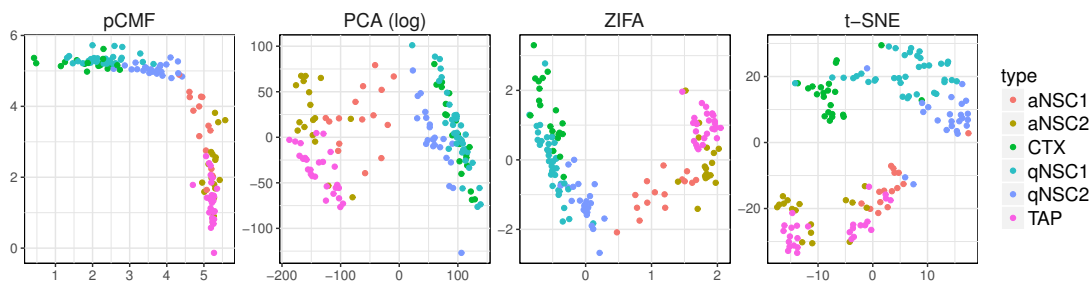
Figure 4: Analysis of the scRNA-seq data from Llorens-Bobadilla et al. (2015), n = 141 cells, p \sim 14000 genes. We pre-selected genes expressed (count > 1 ) in at least 2 cells, with a log-variance higher than 0.5 (as in the original paper). pCMF and t-SNE are applied to raw counts, while PCA and ZIFA are applied to log-transformed counts.
