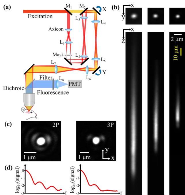
Fig. 1. Three-photon fluorescence microscopy with a Bessel focus. (a) Simplified diagram of our homebuilt three-photon microscope with an axicon-based Bessel module. Flip mirrors M1 and M2 allow switching between Gaussian (yellow path) and Bessel (red path) imaging modalities. PMT, photomultiplier tube. (b) Three-photon images of a 1- \mu\text{m} -diameter red fluorescent bead with different Bessel foci: (left) NA = 0.48, focal length L_1 = 100 mm, L_2 offset = -10 mm; (center) NA = 0.6, focal length L_1 = 125 mm, L_2 offset = -10 mm; (right) NA = 0.72, focal length L_1 = 150 mm, L_2 offset = 0 mm. Post-objective powers: 15.5, 4.9, and 3.2 mW, respectively. Note the different scales for the lateral and axial scale bars. (c) Images of a 0.2- \mu\text{m} -diameter red fluorescent bead taken under (left) two- and (right) three-photon excitation with a Bessel focus of 0.96 NA and axial FWHM of 10 \mu\text{m} (focal length of L_1 = 200 mm, L_2 offset = -10 mm). Contrast was enhanced 7 \times in both images. Post-objective powers: 10 and 16.7 mW, respectively. (d) Signal profiles (obtained from a radial average and plotted in logarithmic scale) of images in (c) . With three-photon excitation the side rings (typical of high-NA Bessel foci) are more effectively suppressed.
