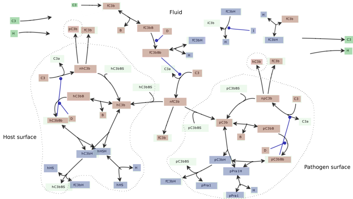
Figure A2: Diagram of all reactions occurring in the C. albicans model. Inflow and outflow are indicated in green, amplification in red and regulation in blue. Starting with the tick-over reaction of C3 into fC3b (top-left), fC3b next associates in fluid with factor B to form the fluid C3 proconvertase (fC3bB). fC3bB is activated by factor D to form the active fluid C3 convertase (fC3bBb). fC3bBb may associate with factor H to form fC3bH, which is cleaved into iC3b by the fluid degradation reactions using factor I (top-right reactions, indicated in blue). If not inactivated, the active fluid C3 convertase (fC3bBb) may convert C3 into C3a and fluid nascent C3b (fnC3b). fnC3b may attach to either host or pathogen surfaces (see section A.1.2), or associate with water to form fC3b (see section A.1.3), which might start the fluid amplification loop again (if not regulated). If fnC3b hits a surface, the same reactions as in fluid may occur, eventually leading to the formation of the active C3 convertase bound to surfaces (pC3bBb and hC3bBb). See also Figs. 1 and 3 in the main text for a schematic visualization of the reactions. The only differences in the reactions on surfaces and in fluid are that factor H may not attach to surfaces unless it is actively acquired by surface proteins (which are pPra1 for C. albicans and hS for erythrocytes) and that a host or pathogen C3b binding site (hC3bBS and pC3bBS) is required for fnC3b to attach to surfaces.
