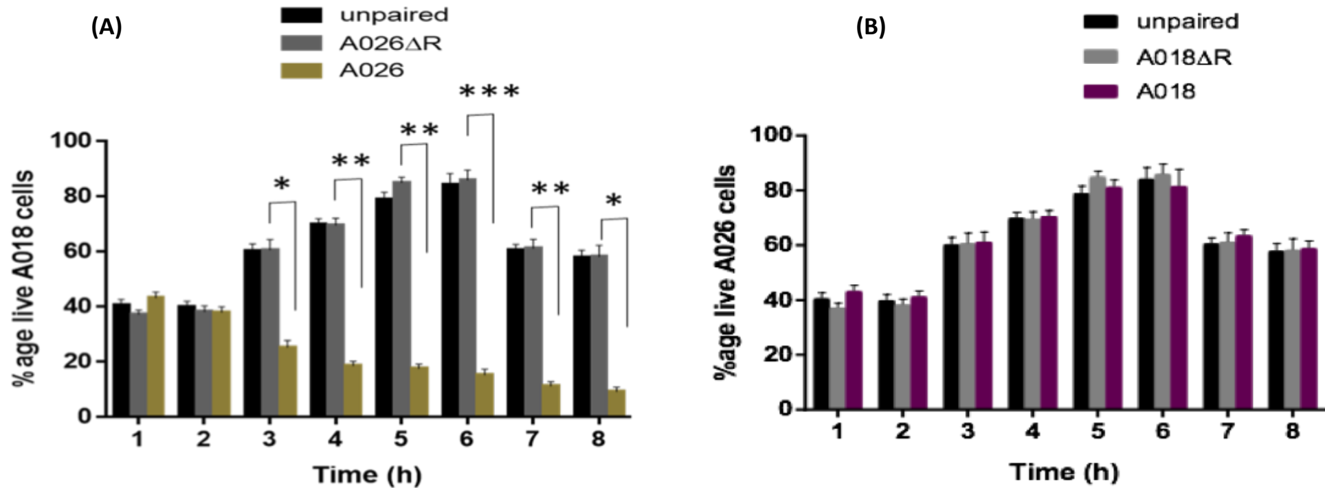
Fig. 2. Planktonic cell competition assay in transwell plates. (A) A018 strain was grown alongside 3 different treatments (A026 wild type, A026ΔR or plain LB), and the percentage of surviving A018 cells in the population was determined over time; (B) A026 strain was grown alongside 3 different treatments (A018 wild type, A018ΔR or plain LB), and the percentage of surviving A026 cells in the population was determined over time. Hourly estimation of the percentages was achieved by staining with BacLight® LIVE/DEAD stain and viewing with a confocal laser scanning microscope. Live cell counts were performed in three fields for each reading. p values \leq 0.005 are significant (Key: *p = 10^{-4} , **p = 10^{-5} , ***p = 10^{-6} ).
