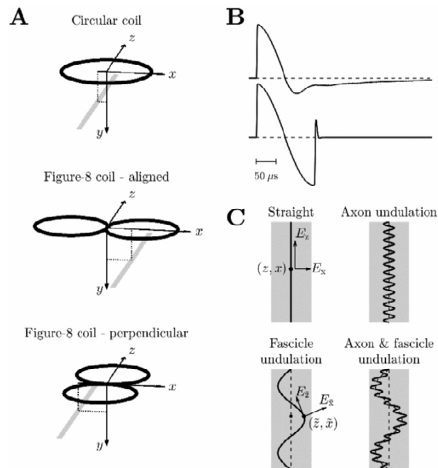
FIGURE 1 Simulation setup. A: Three configurations of magnetic stimulation coils (black) with a nerve (gray) underneath. The coordinate system shows the nerve’s distance to the coil center in the vertical ( y ) and lateral ( x ) directions. B: E-field waveforms of monophasic and half-sine magnetic stimulation pulses, with peak amplitude normalized to unity at pulse onset. C: Four types of axon placement within the nerve trunk. The wavelengths and amplitudes of the undulation are exaggerated for visualization.
