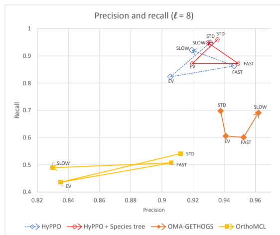
Fig. 7: Precision versus recall values of each method and each dataset for \ell = 8 . Each method has four corresponding points, one for each dataset, and are ordered as follows: Standard - Eventful - Fast - Slow. For example the second point of each path for the analysis of the Eventful dataset.
