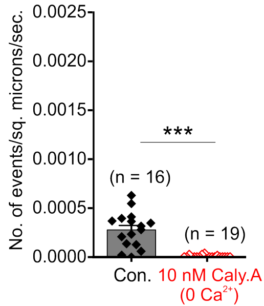
Figure S4. Increase in Ca 2+ flickers with Calyculin A requires external Ca 2+ . Related to Fig 6. Flicker frequency in Control imaging solution and 1-5 minutes after replacing the control bath solution with 10 nM Calyculin A in Ca 2+ -free imaging solution (i.e. standard imaging solution containing 2 mM EGTA and no CaCl 2 ). Bars denote Mean ± sem and each point represents flicker frequency in an individual video. Data are from three experiments. *** denotes p < 0.001 by Kolmogorov-Smirnov test.
