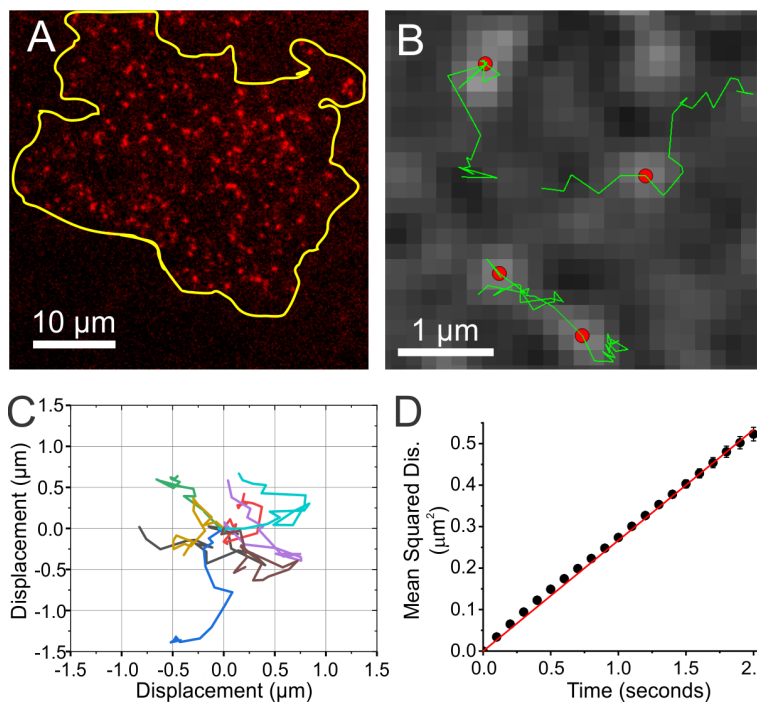
Figure 5. Piezo1 molecules are mobile in the plasma membrane. A. Representative TIRF image of tdTomato fluorescence from mNSPCs harvested from Piezo1-tdTomato reporter mice. Yellow line denotes the cell boundary of the cell. Puncta visible outside the yellow cell line are from neighboring cells. Note the widespread distribution of Piezo1-tdTomato channels over the cell surface. B. Tracking of Piezo1-tdTomato channel puncta imaged at 10 frames per second in live mNSPCs reveals motility of channel puncta. The background image shows fluorescence of Piezo1-tdTomato puncta captured during a single imaging frame. Red dots mark the localizations of the puncta during that frame, and green lines depict the tracks of these puncta over several successive frames. C. ‘Flower plot’ derived by overlaying the trajectories of 10 individual puncta over 1 second after normalizing their starting coordinates to the origin. D. Mean-squared displacement calculated from 6853 Piezo1-tdTomato tracks plotted as a function of time. Error bars represent standard error of the mean. Error bars are smaller than
