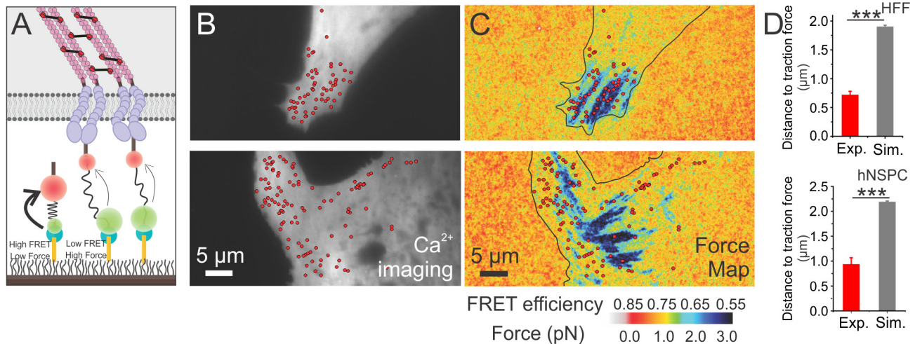
Figure 4. Piezo1 flickers localize to regions of high traction forces, while Piezo channels are motile and widely distributed.
