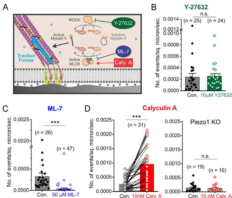
Figure 6. Piezo1 flickers are generated by the action of Myosin II motors. A. Schematic of traction force generation by Myosin II motors. The enzyme Myosin Light Chain Kinase (MLCK, beige and purple) phosphorylates Myosin II (yellow and black) to generate the activated form that binds actin filaments (purple) and produces traction forces (blue arrow). The drug ML-7 inhibits MLCK activity and the drug Calyculin A potentiates MLCK activity, to alter traction force generation by Myosin II. B. Treatment of HFFs by 10 nM Calyculin A increases the frequency of Piezo1 flickers. Left, Paired measurements of flicker frequency in the same fields of view in Control imaging solution and 1-5 minutes after replacement of imaging solution containing 10 nM Calyculin A. Right, 10 nM Calyculin A does not increase \text{Ca}^{2+} flickers in Piezo1-Knockout HFFs. Data are from three experiments; n.s. denotes “not statistically significant” by Kolmogorov-Smirnov test. In all graphs, bar height denotes the mean of the data points, error bars denote standard error of the mean, and the number
