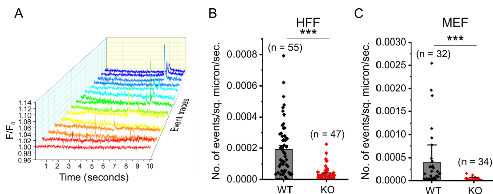
Figure 1. Piezo1 channels generate Ca 2+ flickers. A. Representative Ca 2+ flickers recorded from HFF cells. Traces show fluorescence ratio changes ( \Delta F/F_0 ) from multiple regions of interest, plotted over time and in different colors for clarity. B. Frequency of Ca 2+ flickers in Wildtype HFFs and in Piezo1-knockout HFFs. Bars denote mean \pm sem and each point represents flicker frequency
