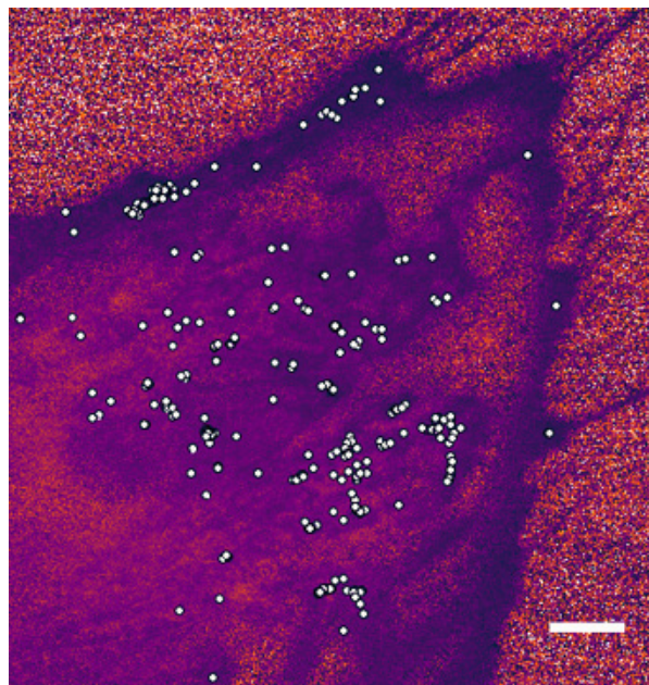
Figure S2. Piezo1 flicker localizations extracted from Movie S1. Related to Fig 2. \text{Ca}^{2+} flickers from HFF Movie M1 were analyzed as described in Fig. 2 and Methods. Scale bar, 10 \mu\text{m} .
