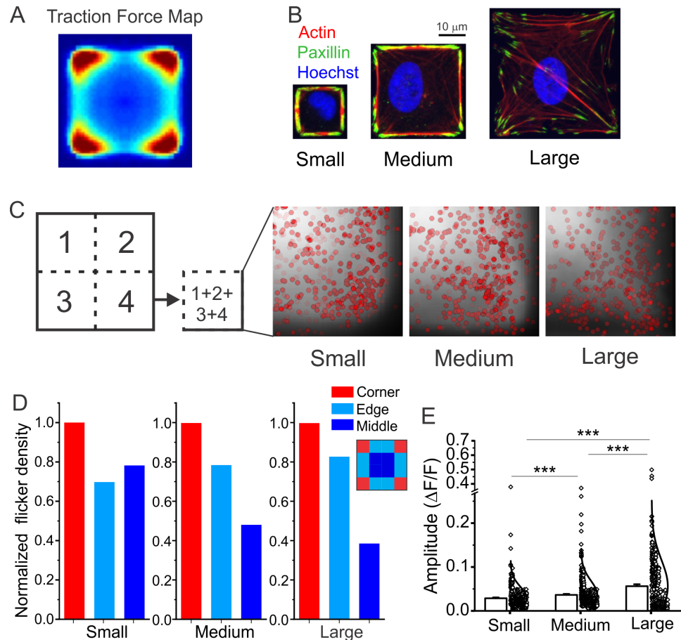
Figure 3. Piezo1 flickers are enriched in regions of cells predicted to have higher traction forces. A. Cells constrained to adopt a square shape on a patterned substrate generate the largest traction forces at the corners (red), lower levels of forces at the edges (cyan) and lowest traction forces in the middle of the cell. The image is reproduced from Holt et al. 2012 under CC BY-NC-SA 3.0 license. B. hNSPCs seeded on square fibronectin islands yield a single square cell per island. Images are representative confocal slices stained for the actin cytoskeleton (phalloidin, red), the focal adhesion zone protein, paxillin (anti-paxillin antibody, green), and the nucleus (Hoechst, blue). Note the larger number of actin stress fibers terminating in focal adhesions as cell spread area increases. Island sizes used: Small, 300 \mu\text{m}^2 ; Medium 1024 \mu\text{m}^2 ; Large, 2025 \mu\text{m}^2 . C. Localizations of Piezo1 flickers within cells seeded on Small, Medium, and Large islands. Each panel shows a quadrant of a Cal520-loaded hNSPC, with an overlay of Piezo1 flicker localizations (red dots); since the square is a symmetric shape, flicker localizations from all four quadrants of cells are displayed on a single quadrant. Total numbers of events represented in panels C, D, E are: Small, 453 events from 7 cells; Medium, 476 events from 7 cells; Large, 426 events from 4 cells. The panels are shown scaled to the same size for ease of comparison. Data were acquired with an exposure time of 5ms (200 Hz frame rate). D. Normalized density of Piezo1 flickers in corner regions (red area in square inset), edge regions (light blue in inset), and middle region (dark blue, in inset) of cells grown on Small, Medium, and Large islands. Flicker density (number of events/ \mu\text{m}^2/\text{s}/\text{cell} ) is normalized to that observed in Corner regions. E. Bar and Data plot of flicker amplitudes ( \Delta F/F ) for events from cells adhering to Small, Medium, and Large islands. Each dot represents an individual Piezo1 flicker event and bars denote the mean of all events for the specified cell size. Piezo1 flickers show greater amplitudes in cells seeded on large islands. *** denotes p < 0.001 by Kolmogorov-Smirnov test.
