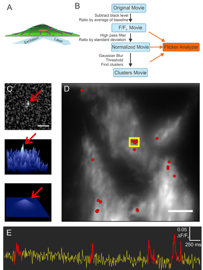
Figure 2. Automated detection and super-resolution localization of Piezo1 flickers. A. Piezo1 flickers are acquired by Ca 2+ imaging with Total Internal Reflection Fluorescence Microscopy (TIRFM). B. Flowchart of the algorithm. The original movie is processed to subtract camera black level and then divided by the average of the first ~100 frames to produce a F/F 0 ratio movie. The ratioed movie is spatially and temporally filtered to increase the signal-to-noise ratio. A clustering algorithm groups supra-threshold pixels into flicker events. C. For every event detected, a 2D Gaussian fit to the fluorescence intensity identifies with sub-pixel accuracy the centroid of the fluorescence, and therefore of the ion channel(s) producing the Ca 2+ signal. Representative images of a 200 μm x 200 μm region showing a processed, filtered Piezo1 flicker event (top, red arrow), a 3D representation of the event (middle) and the Gaussian fit to the event (bottom). Arrow in bottom panel marks the peak of the Gaussian profile that identifies with sub-pixel accuracy the location of the centroid of the Ca 2+ flicker. D. Flicker localizations (red dots) overlaid on an image of an hNSPC to map sites of Piezo1 activity. E. Flicker activity from the region of interest marked in D plotted over time as fluorescence ratio changes (ΔF/F 0 ). Identified flicker events are highlighted in red. Scale bars = 50 μm. See also Movie M2 and Fig. S2.
