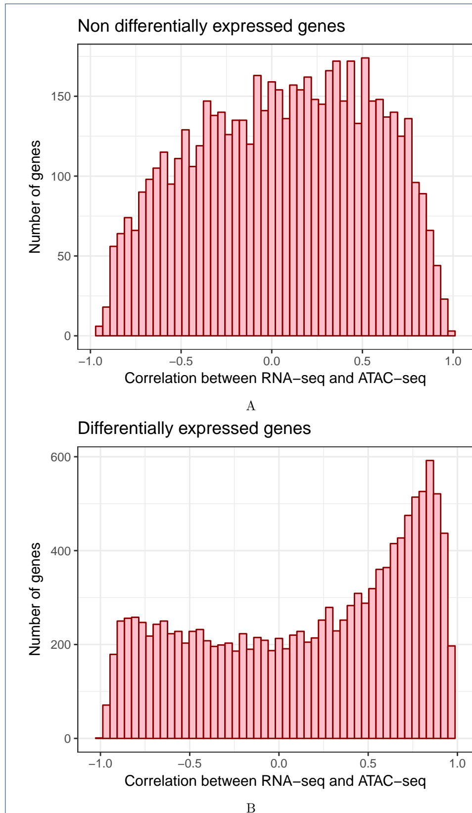
Figure 6 Correlation between gene expression and promoter accessibility in pig. For each expressed FR-AgENCODE gene with an ATAC-seq peak in the promoter region, the Pearson correlation is computed between the base 10 logarithm of the RNA-seq gene expression and the base 10 logarithm of the ATAC-seq chromatin accessibility. The distribution is represented for genes with no significant differential expression between liver and T cells ( A, top ) and for differentially expressed genes ( B, bottom ). The distribution obtained for differentially expressed genes showed an accumulation of both positive and negative correlation values, suggesting a mixture of regulatory mechanisms.
