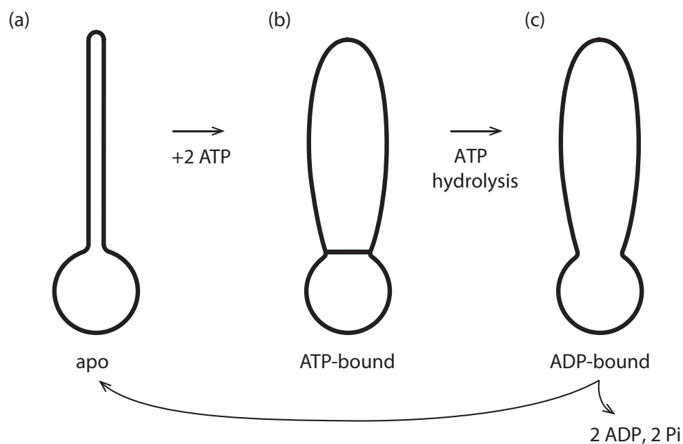
FIG. 3: SMC protein complex states.
