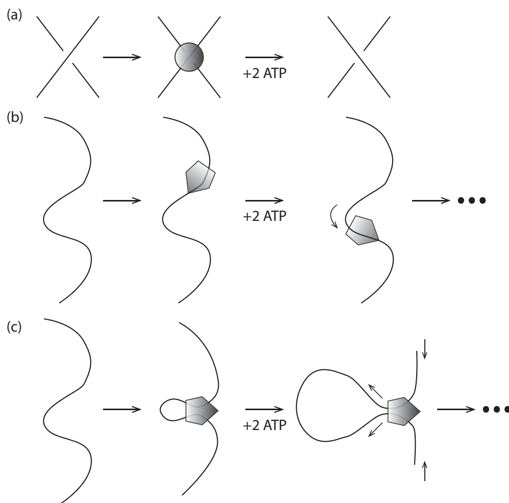
FIG. 1: Two active (ATP-hydrolysis-powered) protein machines responsible for DNA topology control in vivo .
