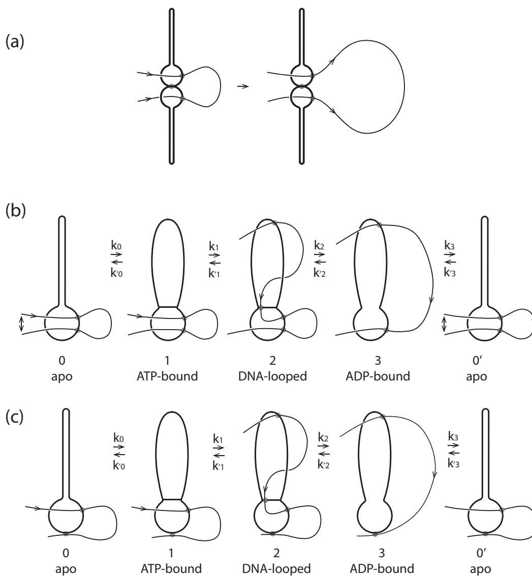
FIG. 7: Models for loop extrusion based on the translocator model of this paper.
