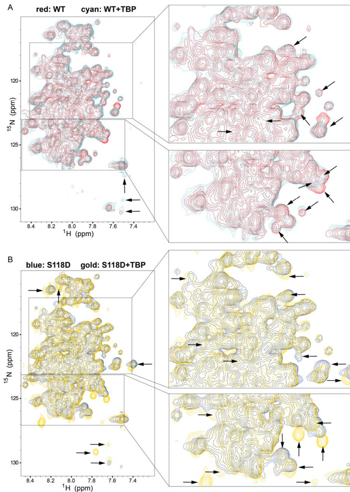
Figure S10. Mutation-induced conformational changes and alteration of coactivator TBP
