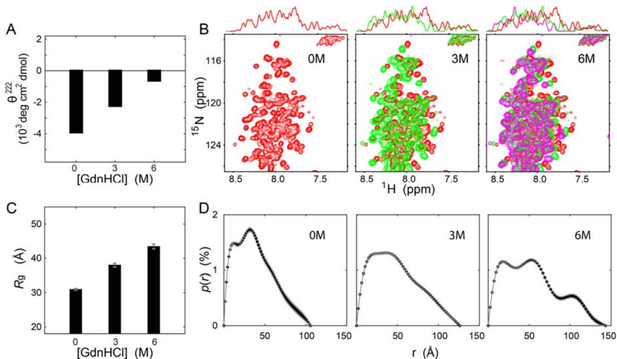
Figure 2. Structural expansion by chemical denaturation.
