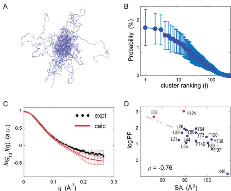
Figure 3. Ensemble-structure construction for the native compact-disordered NTD.
