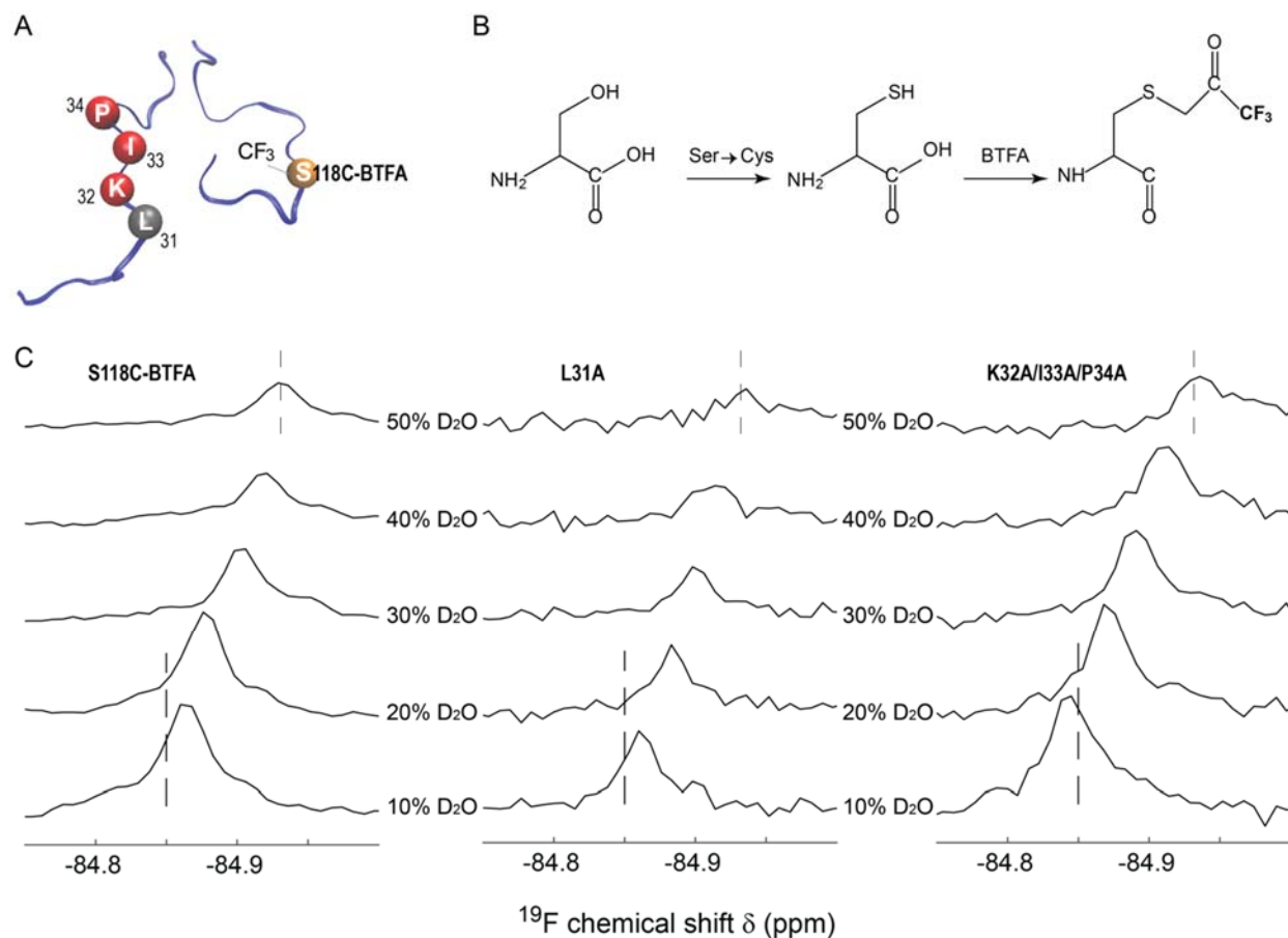
Figure 5. Mutations near residue I33 alter the fluorine-19 chemical shift at residue S118.
