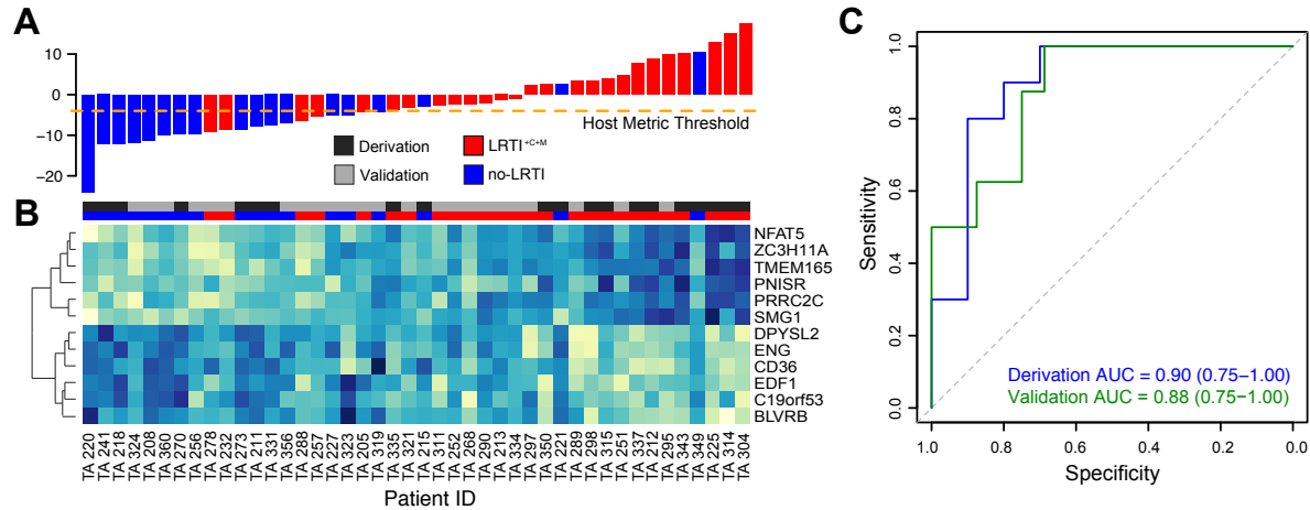
Figure 5. Host transcriptional profiling distinguishes critically ill patients with LRTI (LRTI +C+M ) from those with non-infectious acute respiratory illness (no-LRTI).
