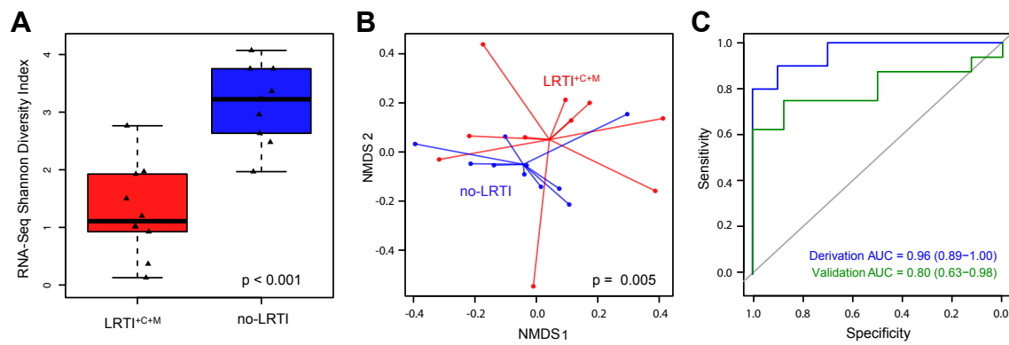
Figure 4. Diversity of the transcriptionally active lung microbiome in patients with LRTI (LRTI +C+M ) versus patients with non-infectious respiratory illnesses (no-LRTI).
