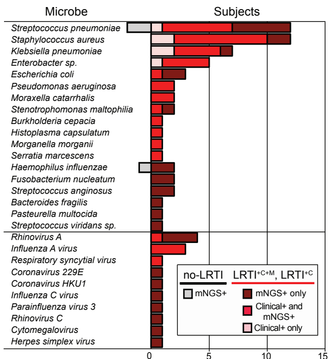
Figure 3. Distribution of respiratory pathogens identified in patients using clinician-ordered diagnostics versus mNGS. For each microbe, the number of subjects from whom that microbe was identified is plotted on the X-axis. Red bars indicate microbes detected by clinician-ordered diagnostics and also predicted as pathogens by either the rules based or logistic regression models. All microbes detected by clinician-ordered diagnostics were detected by mNGS, however pink bars indicate microbes misclassified as negative by either the rules-based or logistic regression models. All microbes identified by clinician-ordered diagnostics and misclassified by either the rules-based or logistic regression models (pink bars) were found in polymicrobial cultures. Additional detail on which model identified each microbe can be found in Figure S2.
