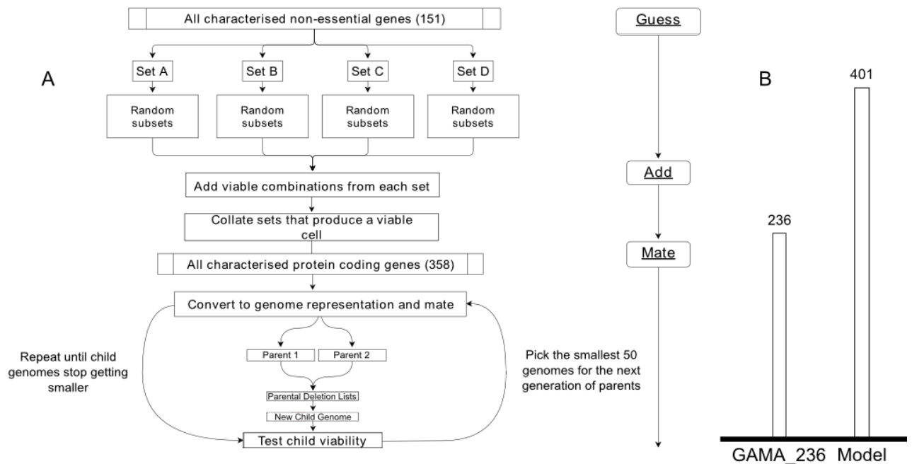
Figure 2 GAMA Method for Genome Design: Example and Results (A) Using the Mycoplasma genitalium whole-cell model to test for genome viability, GAMA reduced the in-silico genome in three stages, Guess, Add and Mate. Guess: split all non-essential genes into 4 groups of roughly 38 genes and randomly pick 400 subsets of greater than 24 genes from each group to knockout in-silico . Add: between two and four of the groups are randomly selected and then one viable knockout combination is taken from each of them. The union of all these knockout sets is taken to create one larger knockout set which can then be tested in-silico . This is repeated 3,000 times. Mate: takes the top 50 smallest genomes that produce a viable cell from the “add” stage and mates them. This mating is done by randomly selecting two parents from the 50 fittest individuals such that smaller genomes are more likely to be picked. A new genome is created by randomly combining parts of the two parent genomes. Finally a number of genes are randomly mutated which creates a child genome to test. One generation of the mate stage consists of 1,000 children and once the viability is known the top 50 fittest individuals is updated to take into account the new results. This is repeated to create new generations of child genomes until no smaller genomes are found for 10 generations. Details of simulations completed and settings are available in the methods and supplementary information. (B) A comparison of genome size between the unmodified Mycoplasma genitalium whole-cell model genome and the GAMA_236 genome.
