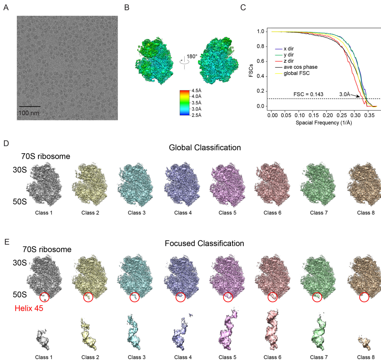
Supplementary Figure 4 – Cryo-EM data for HIV-1 TAR—ribosome fusions. (A) Example raw image collected for TAR-labeled ribosomes. (B) Initial single-model refinement, colored by local resolution and (C) the corresponding FSC curves. (D) Classes generated from global 3-D classification showing a lack of density in the region of helix 45. (E) Classes from focused 3-D classification, with the mask applied to the region of TAR fusion, denoted by a red circle with the corresponding densities of the TAR hairpin in the absence of the ribosome scaffold below.
