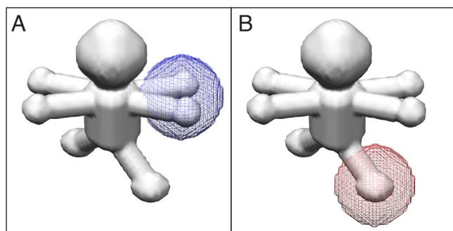
Figure 2 – Application of masks onto regions of an asymmetric unit. Masks were applied either (A) onto the arm/hand region (blue) or (B) the leg region (red) prior to focused classification. Both types of asymmetric units are displayed, showing both orientations of the arm/hand combinations.
