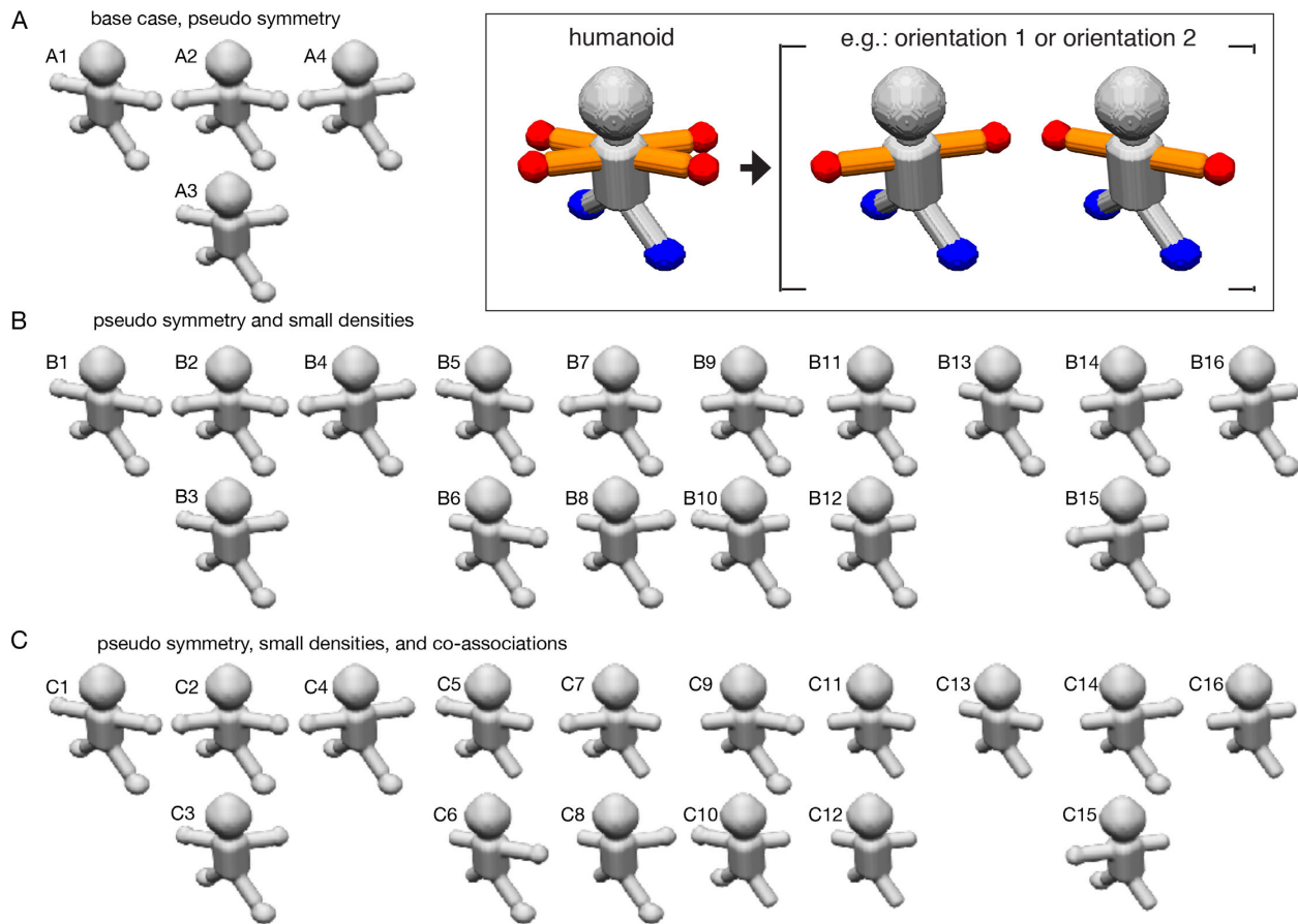
Figure 1 – humanoid datasets and distinct scenarios used to assess focused classification. Different maps used to generate synthetic datasets described by the three scenarios are displayed. In each panel, A-C, two maps which are degenerate and related to one another by a 180° rotation are positioned vertically with respect to one another. The components used to generate the datasets are displayed in the inset, with the heterogeneous elements colored (arms, orange; hands, red; feet, blue). (A) For the base scenario, only the arms/hands are conformationally mobile. Four different combinations of maps lead to a dataset characterized by two different asymmetric units. Maps A2/A3 are related by a 180° rotation. (B) For the second scenario, in addition to the conformational mobility of the arms, the hands can be either present or absent. 16 different combinations of maps lead to a dataset characterized by four different asymmetric units. Maps B2/B3, B5/B6, B7/B8, B9/B10, B11/B12, and B14/B15 are related by a 180° rotation. (C) For the third scenario, in addition to the conformational mobility of the arms, the hands can be either present or absent, but their occupancy is always co-associated with a nearby foot. 16 different combinations of maps lead to a dataset characterized by four different asymmetric units. Maps C2/C3, C5/C6, C7/C8, C9/C10, C11/C12, and C14/C15 are related by a 180° rotation.
