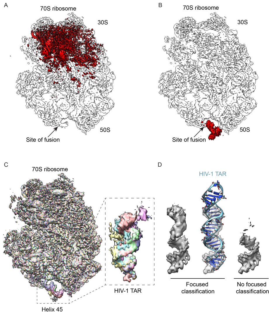
Figure 4 – Experimental reconstructions highlighting the use of focused classification to analyze highly heterogeneous datasets. Bacterial 70S ribosomes containing an HIV-1 TAR element fused into Helix 45 (H45) were used to analyze different classification approaches. (A) Combinatorial pairwise differences between all 8 classes from global classification merged into a single volume to highlight the overall variability. (B) Same as A, but from the result of focused classification using 2-D masks, applied on the region of TAR fusion into H45. In both A-B, arrows denote the site of fusion. (C) Overlaid reconstructions after focused classification, highlighting the differences within the TAR element, but not in the rest of the ribosome. (D) Close-up of TAR reconstruction after deconvolving its mobility through focused classifications (left), shown also with a rigid-body docking of the TAR element into density (middle). A control reconstruction, without focused classification but using the same number of particles, is displayed alongside (right).
