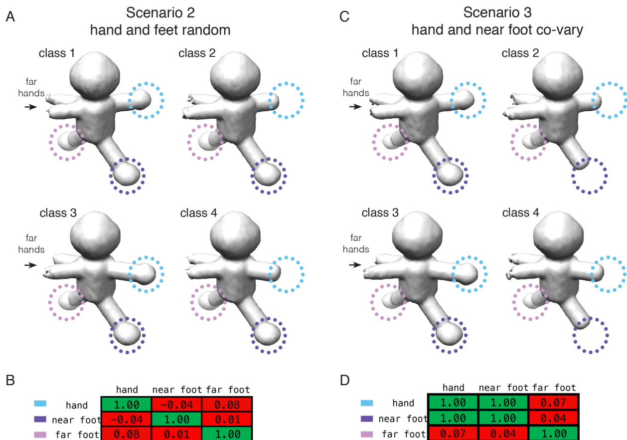
Figure 3 – Evaluation of covariance within two different regions of a reconstructed object. Focused classifications using 2-D masks, applied to an arm/hand region (to the right of body in figure and encompassing both arm/hand conformations), were performed using either (A-B) the dataset for the 2 nd scenario or (C-D) the dataset for the 3 rd scenario, both at an SNR of 0.100. In all cases, four classes were recovered for the different asymmetric units (arms in two positions, each with and without a hand), and are displayed in panels A and C. (A) Volumes recovered from focused classification in the 2 nd scenario, where all components are randomly occupied (control). (B) Normalized covariance matrix describing the relationships between the near hand, near foot, and far foot. (C) Volumes recovered from focused classification in the 3 rd scenario, where the near hand is always co-associated with the near foot. (D) Normalized covariance matrix describing the relationships between the components. Near hand, where focused classification is performed, is circled in blue, near foot is circled in purple, and far foot is circled in pink. In the tables, the values are colored using a gradient: -1 (green, anti-correlated) < 0 (red, not correlated) < 1 (green, correlated).
