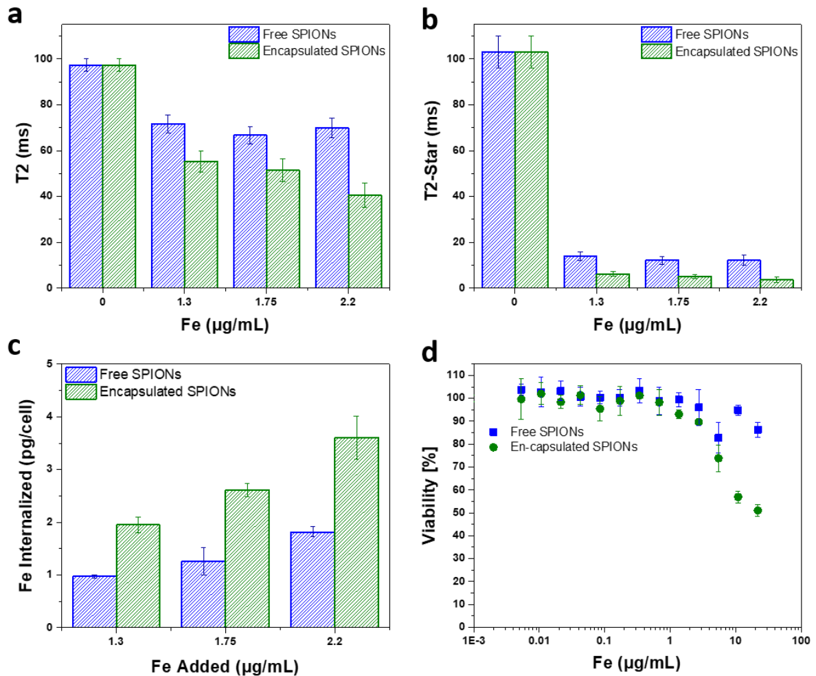
Figure 3: Cell labelling and toxicity of SPIONs. The solution relaxation times ( T_2 and T_2 -star) of the particles are plotted against the concentrations used for cell labelling (a & b). The labelling concentrations of Fe (Fe added to label the cells) are presented along abcisa. Internalization of free and encapsulated SPIONs versus the added concentration of particles used for cell labelling (determined from ferrozine assay) are shown (c). The Fe concentrations of 1.3, 1.75, and 2.2 \mu\text{g/mL} corresponds to the doses of 15, 20, and 25 capsules added per cell. Cell viability against the labelling concentrations of Fe is presented (d). The error bars are the standard deviations of three replicates.
