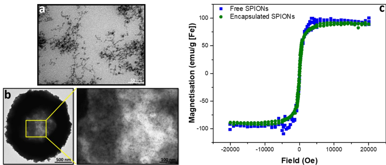
Figure 1: Characterization of free and encapsulated SPIONs by transmission electron microscopy (TEM) and superconducting quantum interference device (SQUID). TEM of free and encapsulated SPIONs is presented in (a) and (b), respectively. SQUID magnetisation curves are shown in (c).
