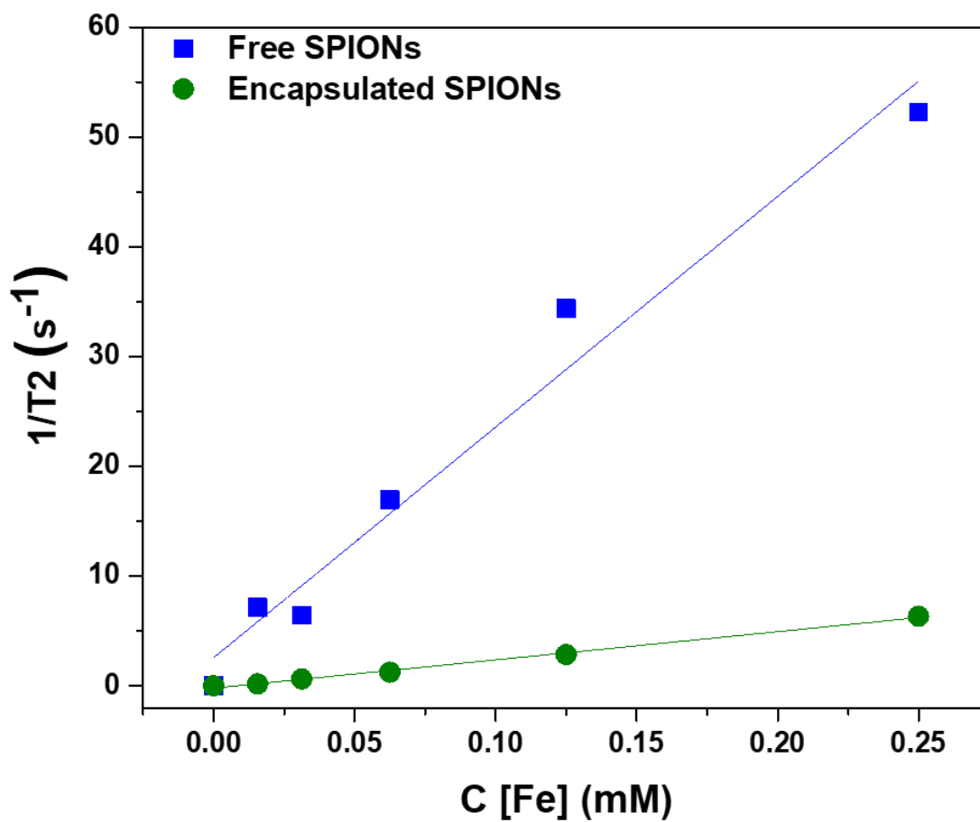
Figure 2: Effect of encapsulation of SPIONs on the solution relaxivity. The water relaxation rates are plotted against the concentrations of particles (in terms of Fe content).
