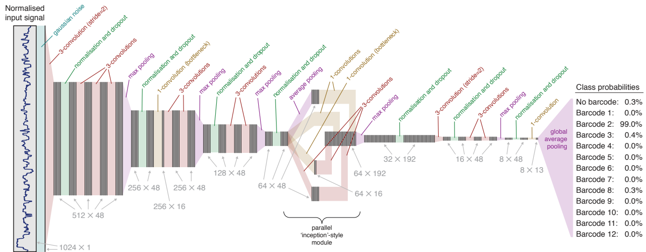
Figure 1. Neural network architecture. Layers in the network are drawn as coloured blocks and data as groups of vertical lines. Data dimensions are shown for each step of the process as data length × filter count . Gaussian noise and dropout layers are only active during network training, not during classification.
