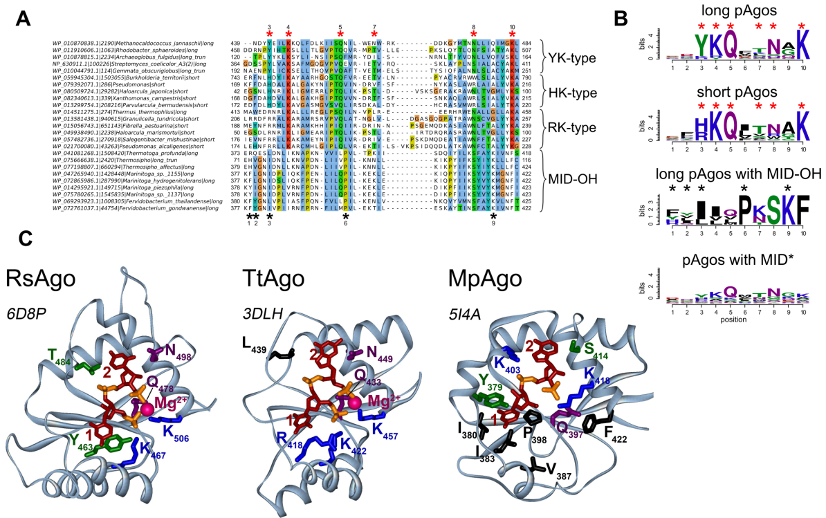
Figure 3. The structure of the 5'-end guide binding motifs in the MID domain. (A). A fragment of the multiple alignment of MID domains of several typical pAgo proteins with different types of the 5'-end guide binding motifs. Red asterisks are the positions of amino acid residues that are involved in the binding of the 5'-P-end of a guide molecule. Black asterisks are the positions of amino acid residues involved in the binding of the 5'-OH-end of a guide in the MID-OH pAgos. MID domains with YK-type 5'-P-end binding motif belong to the long pAgos; MID domains of HK-type belong to the short pAgos; MID domains of the RK-type are characteristic to short pAgos but can also be found in some long pAgos. The multiple alignments were manually edited to bring them in conformity to the secondary structures shown in Fig. 3C. The species names, NCBI taxon_id, the types of pAgos (long, short and long truncated without the PAZ domain) and corresponding accession numbers are shown at the left of the alignment. (B). The sequence logo of amino acid residues involved in the formation of the 5'-end binding pocket for long, short, MpAgo-like pAgos with MID-OH, and long pAgos with MID* domain variants. A combined logo motif including positions characteristic for canonical MID and MID-OH domains is shown. Red and black asterisks are amino acid positions specific for the 5'-P (MID) and 5'-OH (MID-OH) binding motifs, correspondingly. (C). Structures of binary complexes of RsAgo, TtAgo, and MpAgo with guide molecules: 5'-P guide RNA for RsAgo, 5'-P guide DNA for TtAgo or 5'-OH guide RNA for MpAgo. For RsAgo and TtAgo, only residues from the conserved YKQTNK motif are indicated; for MpAgo, MID-OH-specific residues involved in interactions with the 5'-guide end are also shown (labeled with asterisks). PDB IDs are shown next to each structure.
