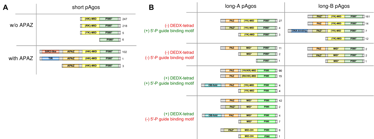
Figure 2. The diversity of domain architecture of pAgo proteins. Various types of domain organization of short (A) and long (B) pAgo proteins are schematically shown. The numbers on the right of each type are the frequency of its occurrence in the redundant set of proteins. Based on the presence of the DEDX tetrad in the PIWI domain and the putative motif 5'-P guide binding motif, all long pAgos can be separated into four types shown here. Green PIWI domains carry the active DEDX catalytic tetrad while turquoise PIWI* domains do not contain the canonical tetrad. Yellow MID domains contain different types of the 5'-end guide binding motif as indicated, while light-brown MID* domains carry substitutions of the crucial amino acid residues in this motif. Orange PAZ domains have full-sized pocket responsible for 3'-end guide binding, while light-brown PAZ* variants do not have the second subdomain. The OB-fold is the nucleic-binding domain SSF50249; the DNA-binding domain comprises Schlafen domain with Alba_2 (PF04326) and lambda-repressor-like domain (SSF47413).
