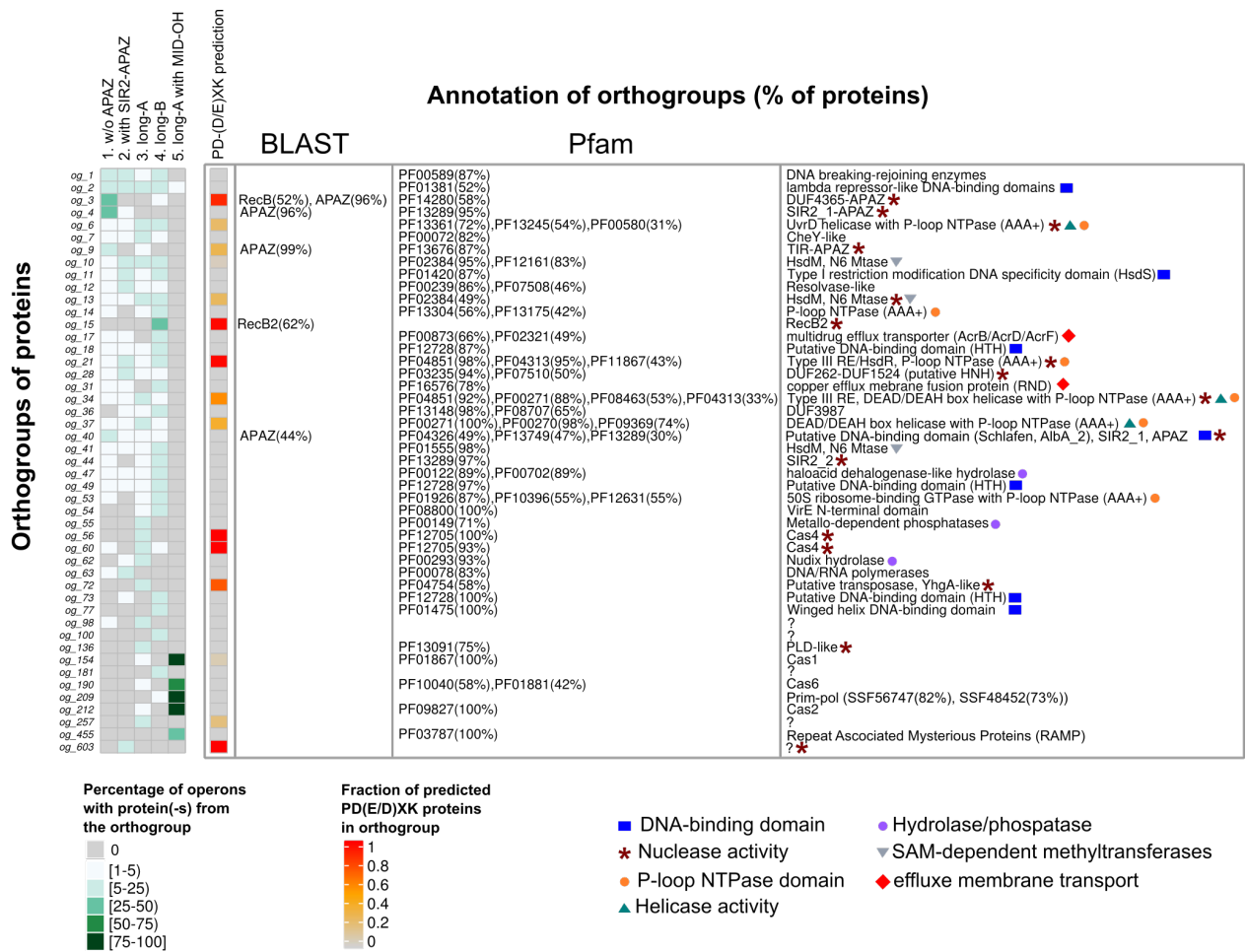
Figure 6. Functional annotations of proteins encoded in pAgo operons. The heatmap on the left shows the percentage of operons for each pAgo group (columns) that have at least one protein from the particular orthogroup (rows). The orthogroups are ordered according to the number of proteins in each group, from the largest to the smallest. The PD-(D/E)XK column shows the fraction of proteins from each orthogroup that are predicted to be nucleases from the PD-(D/E)XK superfamily. The annotation of proteins was performed by BLAST analysis for identification of APAZ, RecB-like, RecB2 domains and by InterProScan with using Pfam and Superfamily databases. Only the Pfam annotation of domains is shown (with the exception of og_209 for which the Superfamily annotation is shown). The percentage in the brackets after the domain name shows the fraction of proteins in the corresponding orthogroup having this type of domain. Only Pfam or Superfamily domains found in at least 30% of orthogroup proteins are shown. The descriptions of domain functions are shown on the right of the panel. Proteins from several orthogroups do not have any known domains and are marked by “?”. After the manual curation of domain functions, several most common functional features were selected, which are shown as colored symbols and described below the table.
