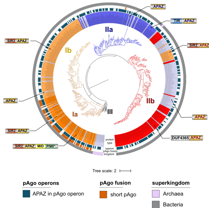
Figure 5. Phylogenetic analysis of APAZ domains. The circular phylogenetic tree of the five groups of APAZ domains. The phylogenetic tree was annotated as follows, from the inner to the outer circles: in the ‘protein type’ circle the APAZ-containing proteins are colored according to their phylogenetic groups and domain compositions, where each type of protein structure is exemplified by the callouts with corresponding domain schemes; isolated APAZ domains in all groups are shown in light blue; the ‘operon’ circle indicates whether the APAZ-containing protein is found in a pAgo coding operon; the ‘pAgo fusion’ circle shows APAZ domains which are fused with short pAgo proteins; the ‘kingdom’ circle indicates the superkingdom to which the corresponding APAZ-containing protein belongs to.
