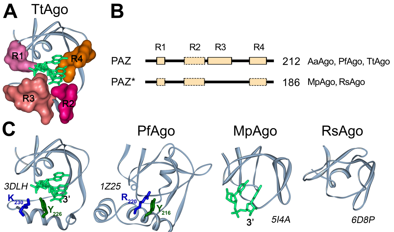
Figure 4. PAZ domains in the pAgo proteins. (A). The structure of the 3'-guide binding pocket in TtAgo (PDB ID: 3DLH). Structural regions R1-R4 forming the pocket are shown in surface representation. (B). A general scheme of the PAZ and PAZ* domain structures in long pAgos. All PAZ domains can have R1, R2, R3 and R4 regions. PAZ* is defined as variants of PAZ lacking full-length region R3. No regions R1, R2 and/or R4 could be detected in multiple alignments of some PAZ or PAZ* variants (shown by broken boxes), but their actual presence need to be tested due to their low conservation. The numbers show how many long pAgos have corresponding domain structure. The pAgos with resolved structures having PAZ and PAZ* domains are indicated. (C). The three dimensional structures of PAZ (TtAgo, PfAgo) and PAZ* (MpAgo, RsAgo) variants in crystallized pAgos and their binary complexes with DNA (for TtAgo) or RNA (for MpAgo) guide molecules. Tyrosin and lysine/arginine residues from R3 in TtAgo and PfAgo, probably involved in guide binding, are indicated. PDB IDs are shown next to each structure.
