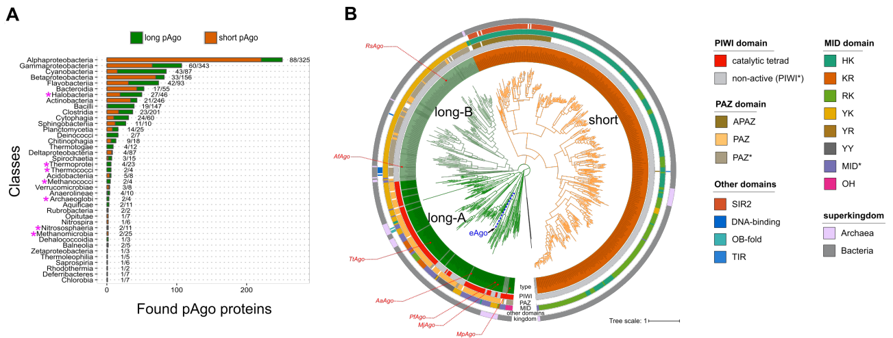
Figure 1. Phylogenetic analysis of pAgo proteins. (A). The numbers of identified short and long pAgo proteins in the classes of Eubacteria and Archaea. Pink asterisks near the clade name indicate the Archaeal classes. The numbers on the right of each bar depict the number of genera encoding pAgos versus the total number of genera with the complete or partially sequenced genomes in the corresponding class. (B). The circular phylogenetic tree of the non-redundant set of pAgos constructed based on the multiple alignment of the MID-PIWI domains. The pAgo proteins were annotated as follows, from the inner to the outer circles: the type of protein, in which long-A pAgos are painted in green (truncated variants without the PAZ domain, light green), long-B pAgos are light-green (truncated variants without PAZ, green), and short pAgos are orange; the type of the PIWI domain, depending on the presence of the catalytic tetrad DEDX; the type of the 5'-end guide binding motif in the MID domain (the first two conserved residues are indicated); the presence and the type of the PAZ/APAZ domains in pAgos; the superkingdom to which the corresponding pAgo belongs to. Biochemically characterized pAgos (or the most similar redundant homologs for RsAgo and TtAgo) with resolved structures are highlighted in red. The scale bar represents the evolutionary rate calculated under the JTT+CAT evolutionary model.
