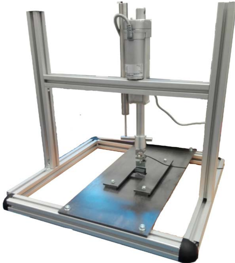
Fig. 02. Measurement station
