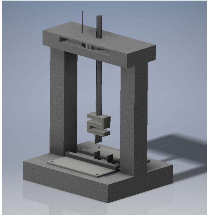
Fig. 01. Initial concept and 3D outline of the machine
