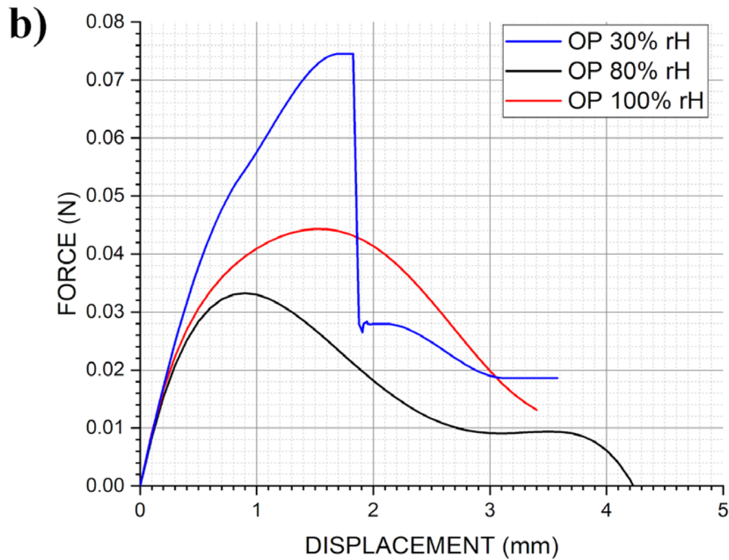
Fig. 06. Example graphs of the force and displacement in various humidity conditions; a - Attacus Atlas , b - Libellula depressa
