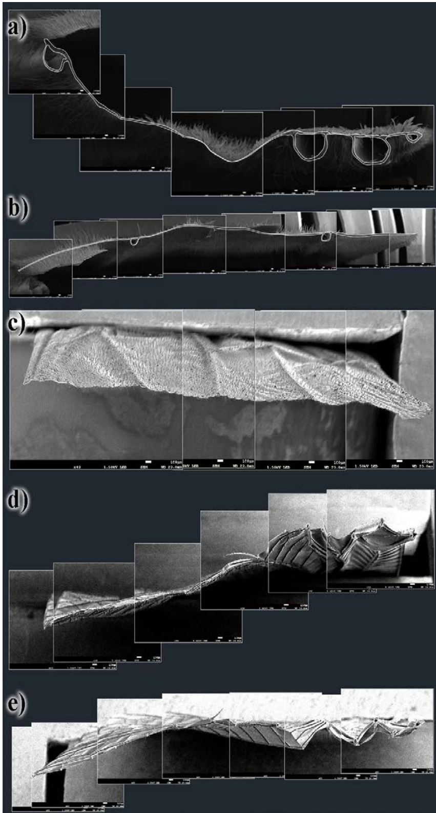
Fig. 08 a) Cross-section of the specimen leading edge of Attacus atlas , b) Cross-section of the specimen leading edge of Attacus atlas , c) Cross-section of the specimen forewing of Vespa crabro , d) Cross-section of the specimen forewing of Libellula depressa , e) Cross-section of the specimen hindwing of Libellula depressa
