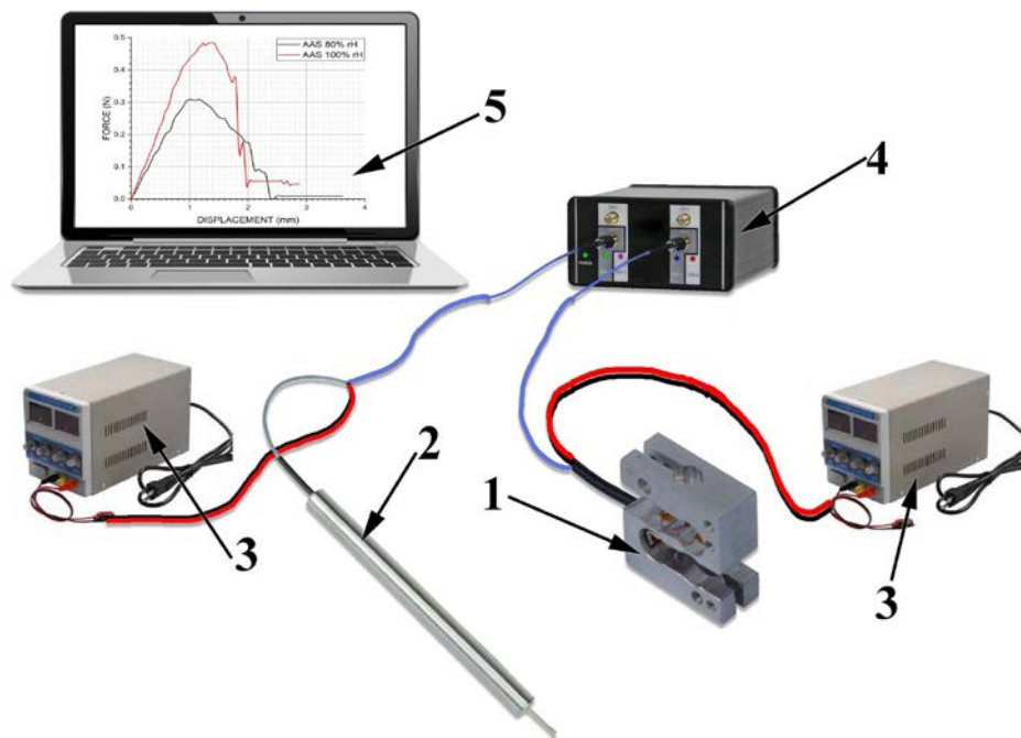
Fig. 03. Schematic drawing of the measurement system. 1 –force sensor, 2 – displacement sensor, 3 – stabilized power source, 4 –signal amplifier, 5 – computer with data acquisition software
