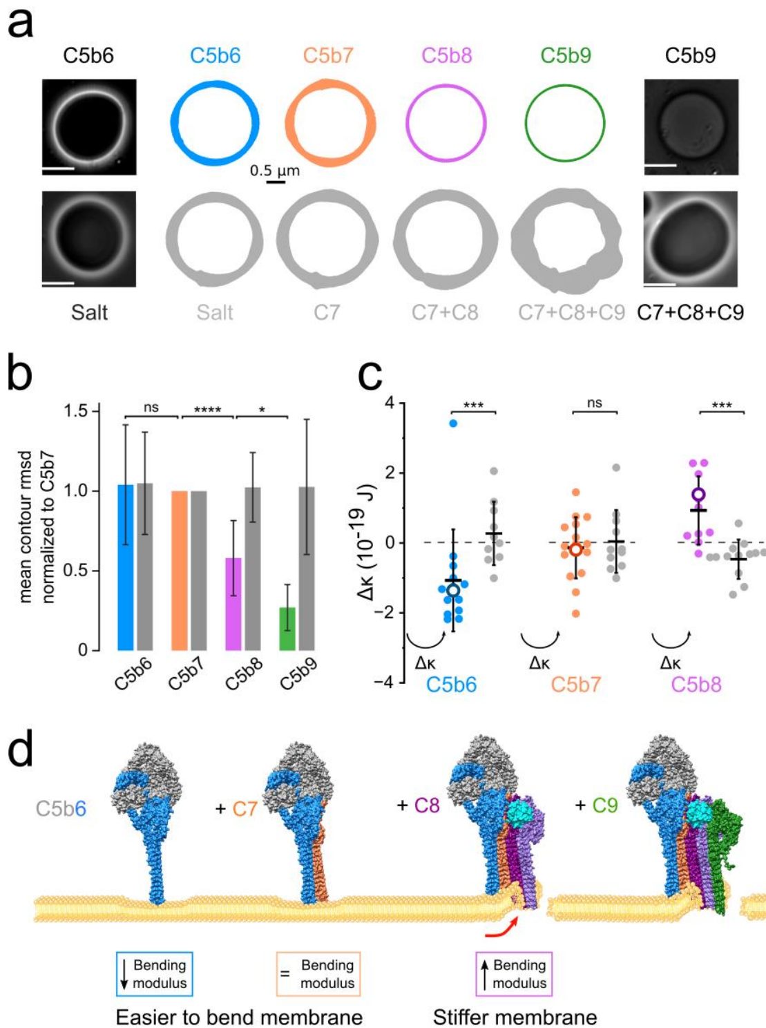
Fig. 4. Flicker spectroscopy informs a biophysical timeline of pore formation.
