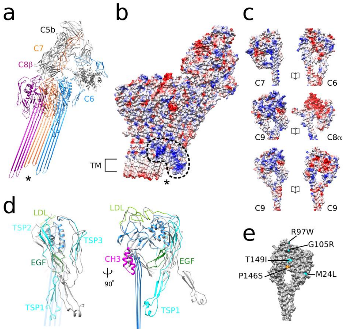
Fig. 2. Structural transitions of complement proteins upon MAC assembly. (a)
