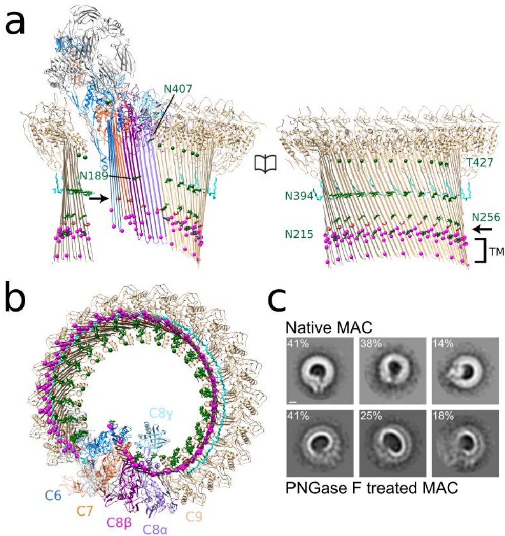
Fig. 3. Glycans provide structural support for a giant \beta -barrel. Molecular model for the open conformation as viewed from within the \beta -barrel ( a ) and from the membrane ( b ). N-linked glycans (green) are shown as sticks (C9:N215, N256, N394; C8 \beta :N189; C8 \alpha :N407). C \alpha carbons of O-linked C9:T427 are represented as green spheres. Backbone trace of C9 C-terminus (res 522:535) is shown as cyan sticks. Disulfide bonds within MACPF domains are red and indicated by an arrow. C \alpha carbons of aromatic residues near the membrane (TM) are magenta spheres. ( c ) Reference-free 2D class averages of negatively stained MAC assembled from de-glycosylated C8 and C9 (bottom panel) show distorted pores on lipid monolayers as compared to native MAC (top panel). Classes are derived from similar particle numbers (native, 706; de-glycosylated, 711). Percentage of particles belonging to each class is indicated. Scale bar, 50 Å.
