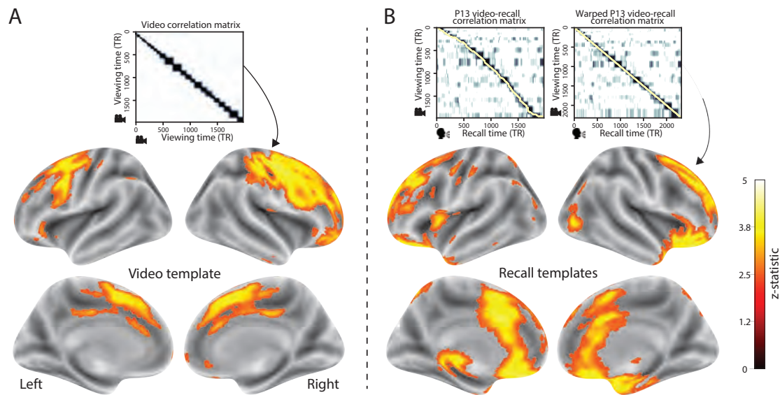
Figure 5: Brain structures that underlie the transformation of experience into memory. A. We searched for regions whose responses (as participants watched the video) matched the temporal correlation matrix of the video topic proportions. These regions are sensitive to the narrative structure of the video. B. We searched for regions whose responses (as participants watched the video) matched the temporal correlation matrix of the topic proportions derived from each individual’s later recall of video. These regions are sensitive to how the narrative structure of the video is transformed into a memory of the video. Both panels: the maps are thresholded at p < 0.05 , corrected.
