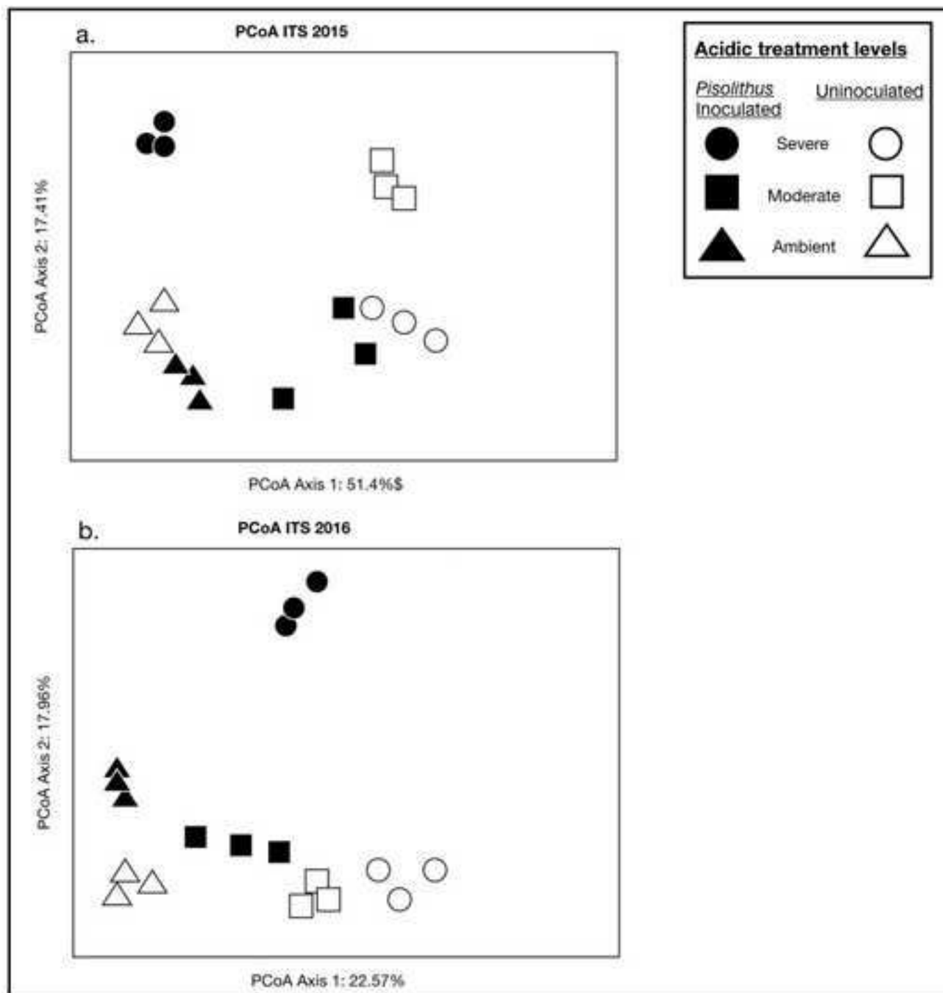
Figure 5. PCoA ITS
