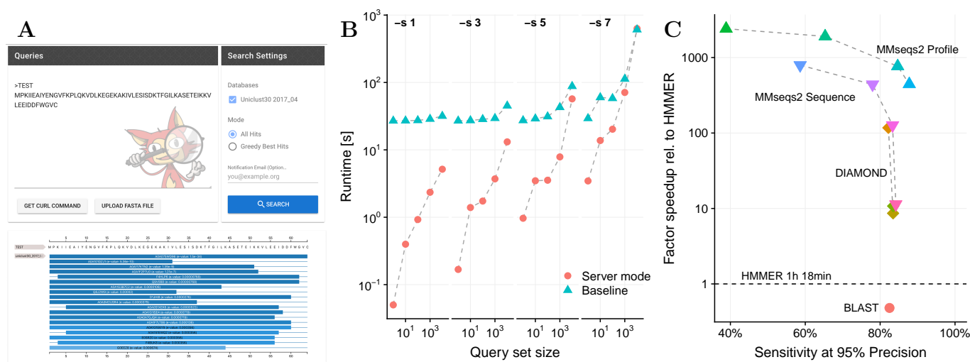
FIG. 1. (A) Screenshots of the search interface and result visualization. (B) Runtime of searches with the baseline MMseqs2 (teal) and the new server mode (red) at four sensitivity settings ( -s ). (C) Domain annotation: Speedup versus sensitivity at 95% precision for MMseqs2 (at four sensitivity settings, -s 1, 3, 5, 7), DIAMOND ( default , --sensitive , --more-sensitive ) and BLAST. HMMER3 matches to Pfam domains are used as ground truth. The speed-ups exclude the times to format the databases.
