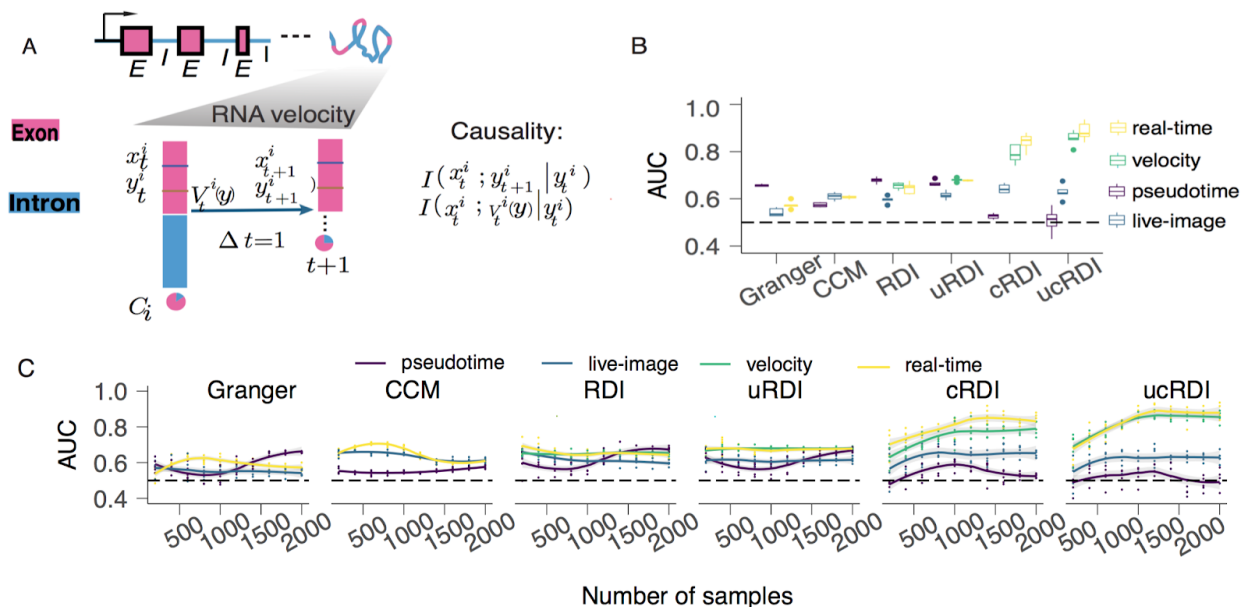
335 Figure 6. Temporally coupled gene expression measurements are necessary for inferring causal regulatory interactions. Four possible types of single-cell time-series datasets, pseudotime (no dynamics coupling across genes and time-points), live-imaging (dynamics coupled for each gene across time-points but not across genes), “RNA-velocity” (dynamics coupled for all gene between two time points measured in each cell) and real-time (dynamics coupled for all gene across all time-points in each cell), are simulated (see Methods for details). 340 (A) Incorporating RNA velocity analysis into Scribe for causal inference. A gene with multiple exons (pink box, E ) and introns (blue line, I ) is transcribed into immature RNA and then spliced into mature RNA, both of which can be quantified by scRNA-seq. See Methods section Benchmarking Scribe with alternative algorithms on inferring causal regulatory 345 network. (B) Dynamics coupling in real time and “RNA velocity” datasets enables Scribe to correctly infer causal regulatory network. Scribe (including four variants, RDI ( k = 0 ), uRDI ( k = 0 ), RDI ( k = 1 ) and uRDI ( k = 1 )) and two alternative causal inference methods, Granger and CCM are used to reconstruct network based on 2,000 data points from each of the four different single-cell time-series datasets. The results from each method are then compared with 350 the known network architecture to obtain the AUC score. Five replicates are performed for each methods. (C) Dependence of causal inference on the number of samples. The same analysis as in A is performed but with downsampled datasets on a sequence from 200 to 2000, incremented by 200, data points (see Methods for more details). RDI: restricted directed information. uRDI: uniform RDI which replaces the biased data distribution with a uniform distribution to remove the 355 dependence of the sample distribution.
