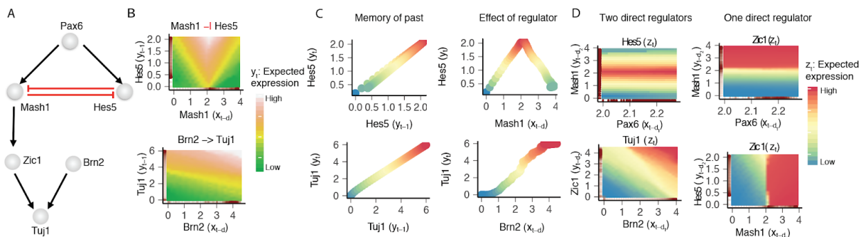
Figure 2: Visualize gene regulations with Scribe. (A) The subnetwork of regulatory interactions visualized by Scribe in panels B-D. See Supplementary Figure 2A for the full network. (B) A causality visualization reveals the information transfer from one gene to another. The horizontal axis corresponds to the regulator’s previous expression with a time lag d while the vertical axis corresponds to the target gene’s very recent past expression. The heatmap color scale corresponds to the expectation of the target gene’s current expression given the target’s its very recent past and the putative regulator expression with a time lag d , or \mathbb{E}[Y(t)|Y(t-1), X(t-d)] . (C) Scatterplots describing relationships of gene regulatory interactions with time delay. (D) A combinatorial regulation visualization reveals the combinatorial gene regulation from two regulators to a target gene. X-axis corresponds to the regulator’s previous expression with a time lag d_1 while y-axis corresponds to another regulator’s gene expression with another time lag d_2 . The heatmap corresponds to the expected value of the target gene’s current expression given both of the regulators’ expressions with the time lags ( d_1 or d_2 ) or \mathbb{E}[Y(t)|X(t-d_1), X(t-d_2)] . For this simulation, all the time delays d , d_1 or d_2 are set to be 1.
