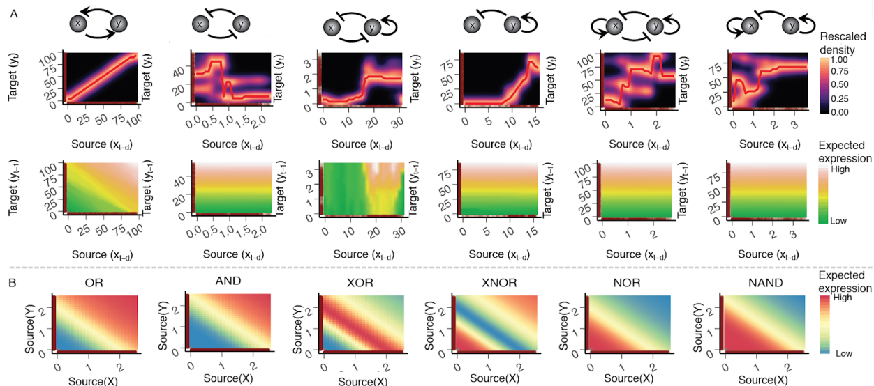
210 Figure 3: Visualizing pairwise interactions from robust two-gene network motifs and combinatorial regulations from common two-input logic gates with Scribe. (A) Visualizing response and causality for two-gene network motifs. Top: robust network motifs from (Ma et al., 2009); middle: corresponding response visualization plots, similar to the DREVI plot reported in 215 (Krishnaswamy et al., 2014) with the difference that we explicitly consider the time-delayed response from the target to the regulator ( P(y_t|x_{t-d}) ) (see methods for more details); bottom: corresponding causality visualization plots. The first node in the motif plot corresponds to the source (x-axis) while the second the target (y-axis). (B) Visualizing combinatorial regulation for six two-input logic gates (OR, AND, XOR, XNOR, NOR and NAND).
