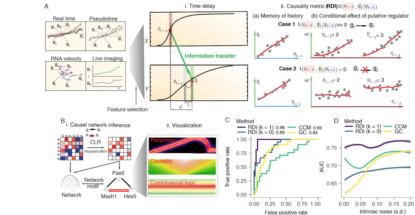
Figure 1: Scribe, a toolkit for inferring and visualizing causal regulations. (A) Scribe detects causality from four types of single cell measurement (“pseudotime”, “live-image”, “RNA-velocity” and “real-time”) datasets with a novel information metric, restricted directed information (RDI). For a putative regulator-target pair, the current state of the target ( y_t ) receives information from the regulator’s previous expression dynamics ( x_{t-d} ) along a time-series trajectory while also having memory of its own intermediate previous state ( y_{t-1} ). Scribe relies on RDI(Rahimzamani and Kannan, 2016) to quantify the information transferred from the potential regulator to the target under some time delay while conditioned over its past on this pseudotime-series data. A gene often has strong memory to its intermediate previous state ( y_{t-1} ) but RDI will only give highly positive causality score from the putative regulator to target in cases where there still is strong relationship between regulator’s history and target’s present conditioning on target’s history (Case 1 vs. Case 2). (B) From pairwise RDI scores, Scribe assembles, refines, and prunes a directed regulatory network. Scribe also incorporates a visualization framework to visualize the response function, causal interaction as well as combinatorial regulation between gene pairs. (C) Receiver Operating Curves or ROC for Scribe, CCM and GC on a linear system. Standard deviation (s.d.) of independent additive noise injected to each gene at each time point and propagate through this system (intrinsic noise) is set to be 0.01. (D) Area Under Curve (AUC) for Scribe, CCM and GC on the non-linear neurogenesis system under different s.d. of intrinsic independent additive noise. See Methods on details of the simulation setup. Note that for panels C/D, k for RDI represents the number of genes to be conditioned for removing indirect causal interactions which is necessary to recover the true causal graph (Rahimzamani and Kannan 2016).
