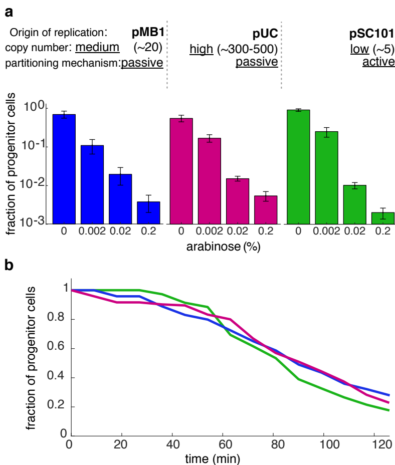
Figure 3 APP in system containing different plasmid origins on the target plasmid. (a) Fraction of progenitor cells as a function of inducer concentration using a target plasmid with the pMB1 (left), pUC (middle) and pSC101 (right) origin of replication as measured by plating assay. Results show that the efficiency of APP can be modulated by varying the amount of inducer. Error bars represent standard deviation of three technical and three biological replicates (b) Fraction of progenitor cells in induced colonies (0.2% arabinose) as function of time, measured by single-cell fluorescence microscopy. Each colony started as a single progenitor cell. Shown are the averages of 12 individual experiments. Each line represents a system with a different origin of replication on the target plasmid: pMB1 (blue), pUC (purple), pSC101 (green).
