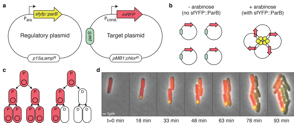
Figure 1 Asymmetric plasmid partitioning in E. coli . (a) The APP network consists of two plasmids: the regulatory plasmid containing parB under the control of an arabinose inducible promoter and the target plasmid containing the parS sequence and the gene encoding red fluorescent protein. (b) In the absence of arabinose (left), there is no ParB, so target plasmids are free to diffuse around the cell. However, when arabinose is present (right), ParB binds the parS sequence on the target plasmid, forming a nucleoprotein complex that gathers all copies of the plasmid together. (c) At the population level, target plasmids segregate normally in the absence of arabinose (left) and all cells remain progenitor cells (denoted by “P”). Upon induction (right), progenitor cells begin to asymmetrically divide, giving rise to daughter cells (denoted by “D”). Note that, during induction, daughter cells are free to propagate, while the number of progenitor cells should remain constant. (d) Time-lapse fluorescence microscopy of cells undergoing asymmetric plasmid partitioning. Shown at time t=0 is a single progenitor cell that is in the presence of arabinose. A nucleoprotein complex quickly forms (yellow punctum), and subsequent daughter cells lose the target plasmid. The inherited red fluorescent protein in the daughter cells quickly decays through dilution and proteolysis.
