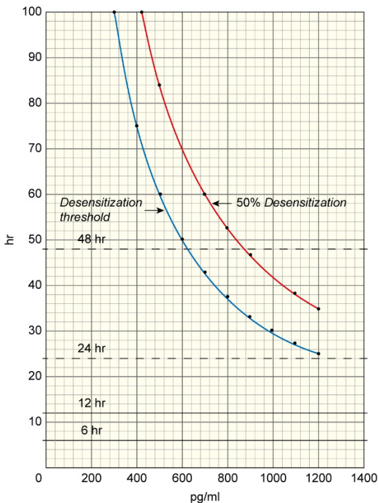
Figure 4. Oxytocin Override Desensitization Threshold and 50% Desensitization Level as Functions of Pitocin infusion time T during labor and Oxytocin Override Concentration C , where CT = D = 1.8\text{E}6 ( \text{pg}\cdot\text{min} )/ \text{ml} for the Oxytocin Override Desensitization Threshold.
