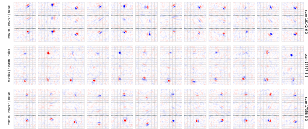
(a) Receptive fields
