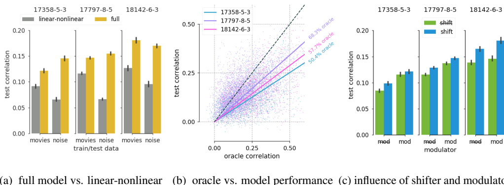
Figure 2: Performance of the model. (a) Single trial correlation of the model prediction with the neuronal responses across neurons for the full recurrent model and a spatio-temporal linear-nonlinear model equipped with a shifter and modulator. Error bars mark 95% confidence interval. (b) Model test correlation against oracle correlation, which represents an upper bound of the achievable performance bases solely on the stimulus. The percentage of oracle was computed from the slope of a linear regression without offset. (c) Influence of the single network components on the prediction performance.
