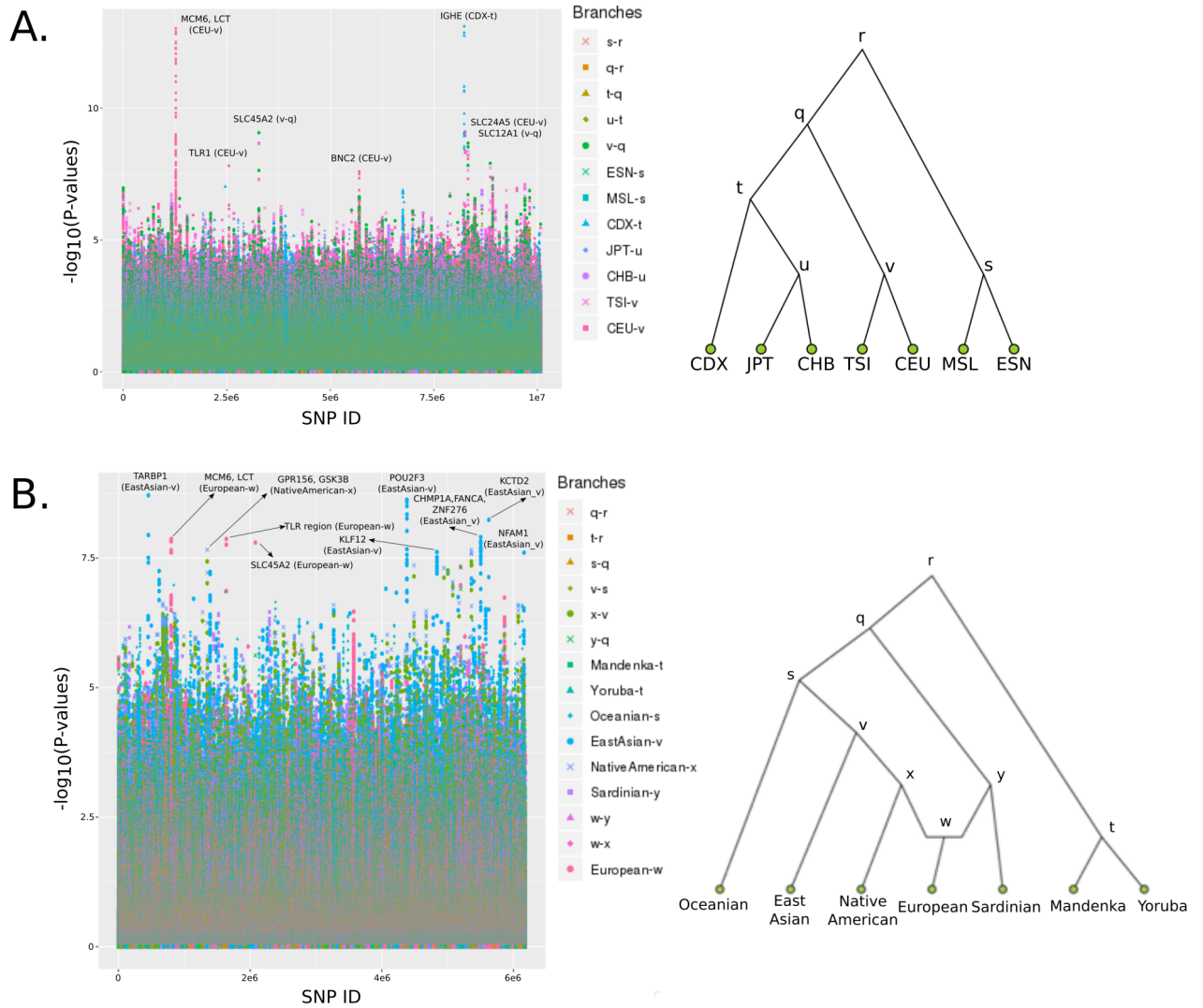
Figure 3: Results from running GroSS on human genomic data. A) Population tree including panels from phase 3 of the 1000 Genomes project. B) Population graph including imputed panels from the Human Origins SNP chip data from Lazaridis et al. (2014).
