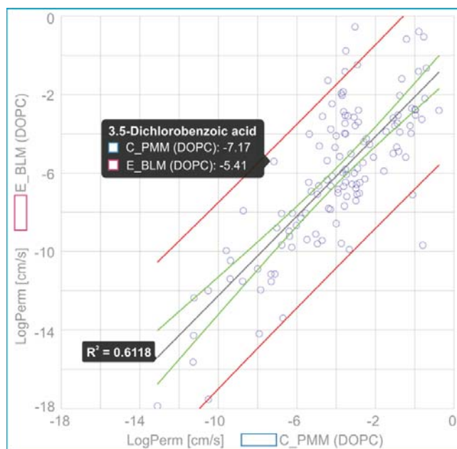
Figure 6. Comparison of permeability coefficients obtained from experimental BLM method and theoretical PerMM model. The figure was manipulated externally from downloaded data to add linear regression line shown in grey with confidence interval shown in red and prediction interval, in green. Confidence interval was set to 95%.
