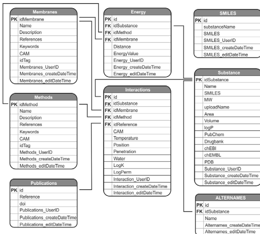
Figure 2. Scheme of MolMeDB database.
