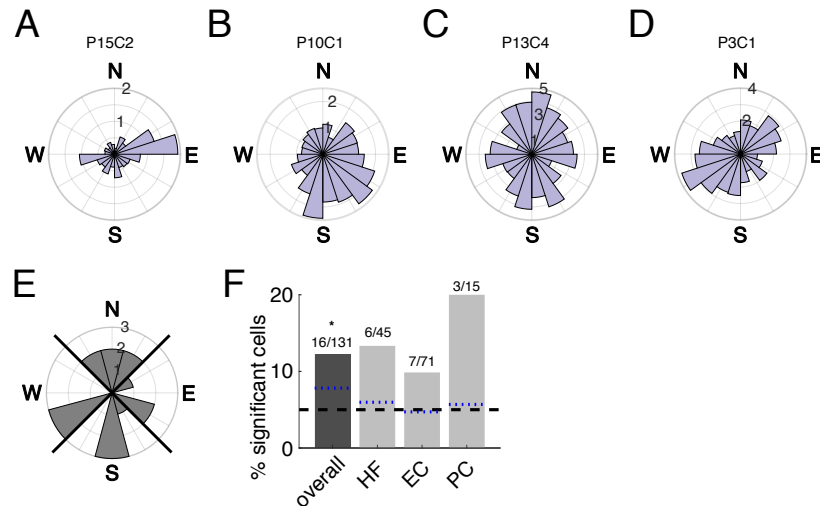
Figure 3: Neural activity related to the subject's heading. Firing rate by virtual heading direction ( N =“north”, E =“east”, S =“south”, W =“west”) for example cells significantly modulated by heading direction. A) Circular histogram of firing rate by heading direction for example cell from Patient 15, in the left hippocampus, significantly modulated by heading direction ( p = 0.026 ). Firing rate is indicated with numbers on the concentric circles. B) Example cell from Patient 10, in the left parahippocampal cortex, significantly modulated by heading direction ( p = 0.005 ). C-D) Two more significant heading-modulated cells, both in the left hippocampus (from Patient 13; p = 0.0315 , from Patient 3; p = 0.003 ). E) Circular histogram of preferred heading directions for each significant heading direction cell. Counts indicate number of cells with that preferred direction. Black diagonal lines indicate NESW quadrants. F) Percentage of significant heading-modulated cells by region. Symbols above the bars indicate p -values from a one-sided binomial test for each proportion (** p < 0.01 , * p < 0.05 , + p < 0.1 ). The black dashed line represents the 5% false positive rate, and the blue dotted lines are the lower 95% confidence interval from the one-sided binomial test for each bar.
