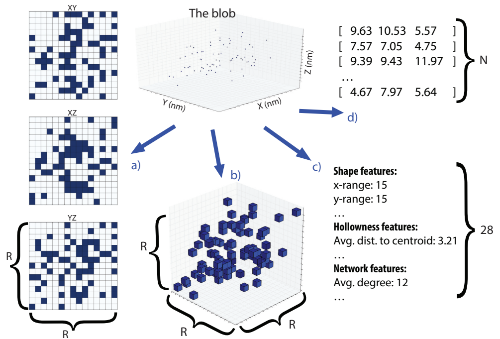
Fig 3. Possible input representations of a point cloud with range R and number of points N . a) Three projections of the 3D point cloud onto 2D planes. Requires 3 \times R^2 values to represent. b) A voxel representation. Requires R^3 values to represent. c) Hand crafted features. Requires 28 values to represent d) A point cloud. Requires 3 \times N values to represent. Where N is the number of points per blob
