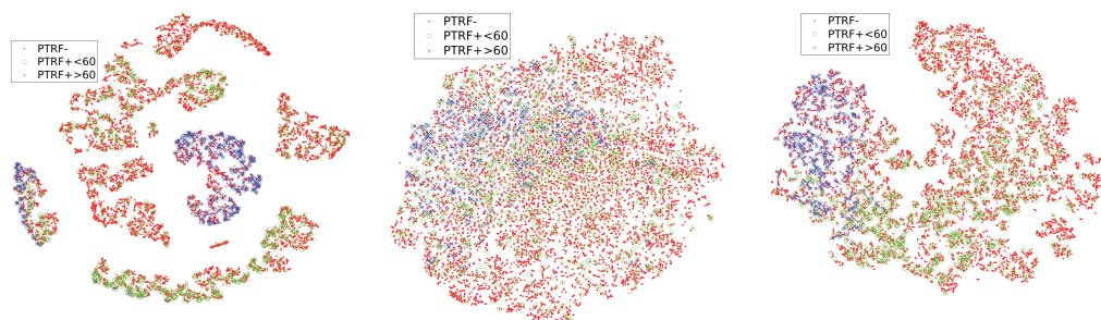
Fig 5. 2D t-SNE visualization of the projected feature space from the various data representations used for identifying the Cav1 blobs. We visualize the projection of high-dimensional feature space into 2-dimensional space using t-SNE from the multi-view CNN, point cloud - PointNet, and hand crafted features. Every point in the t-SNE plot represents the projected features of a blob. The red, green, and blue points represent the projected features of the PTRF-, PTRF+ < 60, and PTRF+ \geq 60 blobs respectively.
