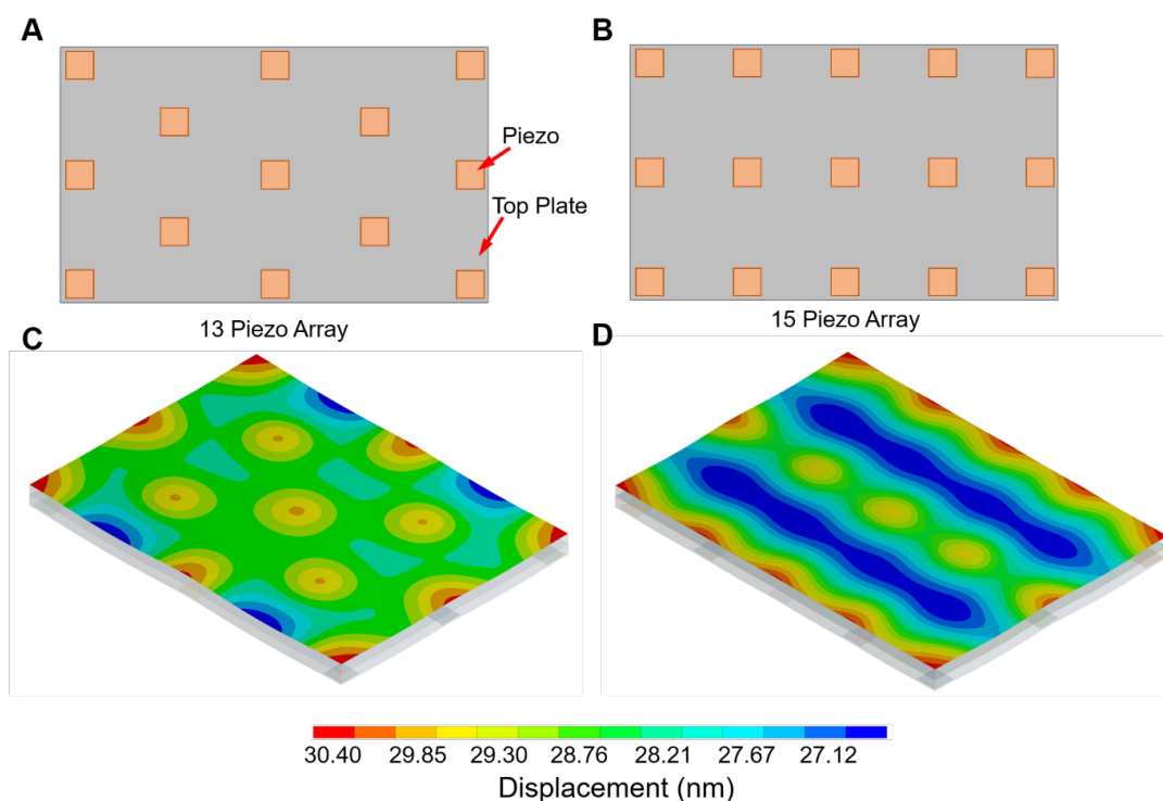
Figure 1. FEA analysis was performed in ANSYS workbench 17.1 to determine the harmonic response at 1 kHz on the thirteen and fifteen piezo array top plate arrangement. (A) Diagram of thirteen piezo array (B) Diagram of fifteen piezo array (C) Predicted nanoscale displacement of thirteen piezo array at 1 kHz (D) Predicted nanoscale displacement of fifteen piezo array at 1 kHz.
