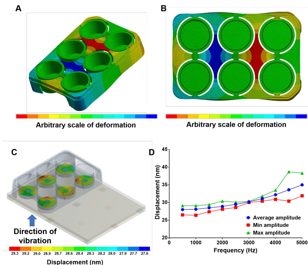
Figure 3. (A) and (B) show the mechanical response of the PP 6-well plate at its 12th mode (1037 Hz). Even though there are resonant modes in the bioreactor operating window, the resulting large scale displacement is confined to the frame and the wells themselves are unaffected. (C) Harmonic response analysis of combined 6-well plate and bioreactor top plate. (D) Frequency response of combined 6-well plate and bioreactor top plate component with fixed 30 nm displacement applied to the piezo bonding points.
