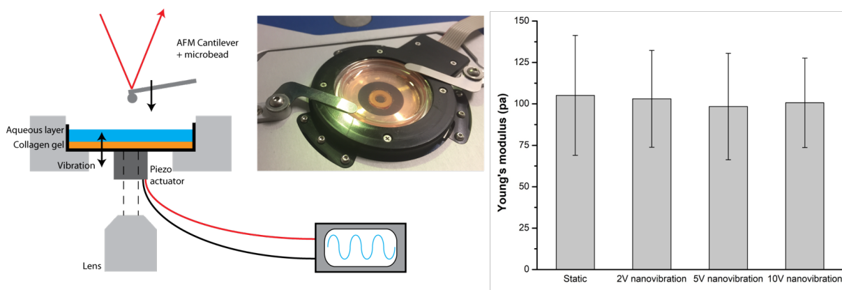
Figure 7. AFM measurement of collagen gel during nanovibration. (A) A vibrating piezo actuator was attached to a Petri dish containing collagen gel with an AFM cantilever being used to measure any changes in gel stiffness during vibration. (B) Young's modulus was assessed via AFM for collagen samples which were nanovibrated at three different piezo amplitudes. Data are mean \pm SD ( n > 30 ).
