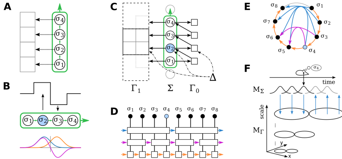
Figure 6: On-line learning of the Transition Scale-Space with temporal buffering. (A) Consecutive activation of symbols \sigma_i \in \Sigma induces a linked list in time (green box). This preserves temporal (small green arrows) and spatial structure (indicated as arrows to discrete spatial areas). (B) Receptive fields of transitions for temporal integration as Haar wavelet (discrete case, top row) and Difference of mean-shifted Gaussians (biologically plausible representations, bottom row) on scale 0. Temporal transition start and end indicated as black arrows. (C) A transition on scale s > 1 (left) needs to associate its on-center (black solid box) with multiple symbols of \Sigma (middle). To keep their spatio-temporal structure, they are activated in sequence (green box) by iterating scale s = 0 of the scale-space (right). Black dashed box indicates spatial off-center (partial area only for visual purposes). (D) Simplified depiction of (C) for three scales. (E) The temporal buffer can be implemented as circular buffer. (F) Multi-scale illustration for biologically plausible receptive afferents. For further explanations for each panel, see Subsection 3.5.
