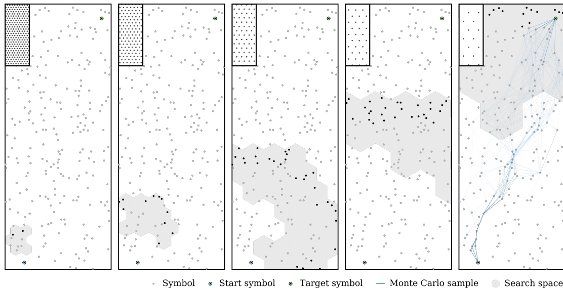
Figure 10: Searching a viable sequence from start (lower left) to target (upper right) using ascending mode. Each scale is expanded at most 3 times before ascending to the next scale (panels from left to right), until the highest scale is reached. Note that, in contrast to Figure 9, here the gray area depicts all images of spatial transitions that were expanded during search, and not the solution space. Black dots indicate the last symbols that were active on a scale before ascending to the next scale or when the target was encountered. The rightmost panel includes Monte Carlo samples (blue lines), generated using the backtracking algorithm. Distribution of transition encoders is shown in the small inlays in each panel, and was precomputed according to prior theoretical results presented in Waniek, 2018. Symbols (gray dots) were distributed randomly on the input space.
