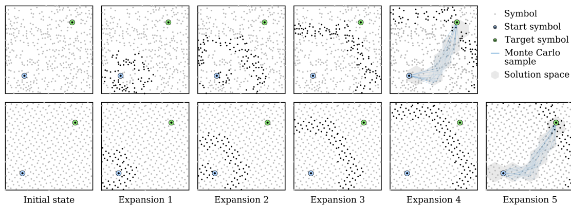
Figure 8: Propagating wave during expansion from start to target in a square environment. Top row shows results for randomly distributed symbols (gray dots), bottom row for symbol coordinates according to the Hammersley point set. Transition encoders were placed regularly on a hexagonal lattice (not shown) due to results presented in Waniek, 2018. Final panels include the solution space (gray area) and 300 Monte Carlo samples (blue lines). The solution space are all those images of transition encoders which contain symbols that are on a shortest path from goal to target. See Appendix E for results in a non-Euclidean space. symbolic sequences were computed using backtracking and randomly selecting a parent during each backtracking step.
