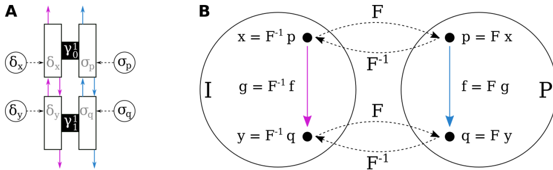
Figure 14: Transitions, grid cells, and category theory. (A) Visualization of grid cells according to scale-space MTS that learn transitions from symbols \delta_x to \delta_y , while also learning transitions from \sigma_p to \sigma_q . (B) Commutative diagram of category theory, in which a morphism g maps objects x to y in a category \mathbf{I} , a morphism f maps objects p to q in a category \mathbf{P} . The morphisms and objects are linked by a functor F that preserves structure of the categories.
