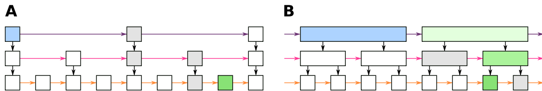
Figure 13: (A) A skip list is a multi-layer linked list data structure (Pugh, 1990). Elements of the list must be ordered. Higher layers have fast lanes to skip over elements. Given a start (blue), searching an element (green) in a skip list starts in the highest layer. Skip links are followed until an element on the corresponding layer is found which is larger than the target. Then, the search is continued on a lower level (see gray boxes). (B) In contrast to skip lists, interval skip lists (Hanson, 1991) store intervals in higher layers. Searching an element is similar to skip lists, but tests if the target element is in an interval (indicated by larger boxes), and subsequently drops down in the hierarchy. Interval skip lists are related to segment trees (see de Berg et al., 1997).
