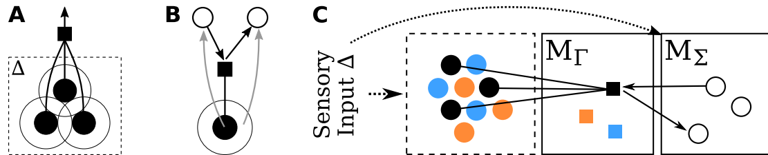
Figure 1: Conceptual overview of the hippocampal-entorhinal Multi-Transition System proposed in (Waniek, 2018). (A) A spatial transition bundle (black square) learns as many transitions as possible to maximize storage capacity of its dendritic tree (dense packing of on-center and off-surround circles). The input space on which this is performed is denoted \Delta , and on-center areas are called spatial symbols \delta_i \in \Delta . (B) A spatial transition bundle \gamma learns feasible transitions in a suitable input space and conveys this information to place cells \delta_i, \delta_j (white circles). (C) Learning a dense coverage of \Delta requires multiple spatial transition bundles (grid cells; colored squares) in memory M_\Gamma . These bundles convey spatial transition information to symbols \sigma_i (place cells; white circles) of memory M_\Sigma . Note that not all connections from transitions to bundles are depicted to improve clarity of the illustration.
