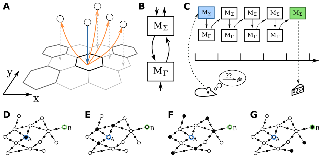
Figure 2: (A) Discrete Voronoi clustering on a suitable input space (indicated by the x - y axes) with absolute WTA dynamics yields hexagonal fields. A spatial transition (black hexagon) associates with all symbols that are co-active with its domain (circle with blue arrow) during exploration, and learns transitions (orange arrows) to symbols in its image (circles with gray dashed arrows). Dark gray, periodically repeating hexagons indicate the bundle to which the spatial transition belongs. (B) Memories of a MTS are recursively connected, shown only for M_\Sigma and M_\Gamma . (C) Given activation of a starting symbol (indicated by blue color of M_\Gamma ) on a linear track that was discretized into bins (black arrow with vertical bars), mentally traveling to a target involves recursively activating M_\Sigma and the transition memories (only M_\Gamma shown here) until the target symbol is active in M_\Sigma (indicated by a green box). (D-G) Propagating wave of activity (black circles) in a graph when searching if a connected path exists between symbols A and B . Each edge involves a spatial transition, indicated by a small black box.
