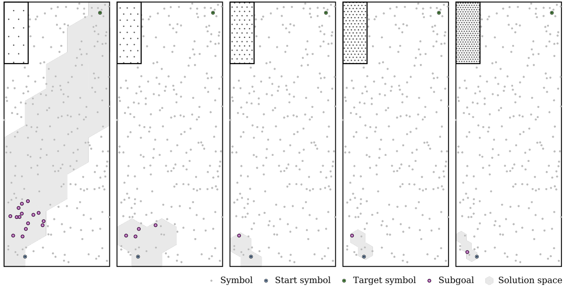
Figure 9: Searching a viable sequence from start (lower left) to target (upper right) using descending mode in a space with randomly sampled symbols (gray dots). The search from start (blue symbol) to target (green symbol) starts on the highest available scale (left panel) and generates sub-goals (magenta symbols). Gray area displays the solution space, which consists of all images of spatial symbols that were expanded and contain trajectories with equal distance. The solution is then refined using finer scales, which compute only partial solutions to the sub-goals from the next higher scale (remaining panels). Distributions of transition encoders are shown in the small inlays in each panel, and were precomputed based on results presented in Waniek, 2018.
