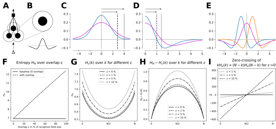
Figure 4: (A) Each spatial transition bundle receives afferents from a spatially modulated input space \Delta and densely packs on-center and off-surround receptive fields. (B) Each receptive field can be treated independently and is modelled as Difference of Gaussians (DoG). (C) Bottom-up construction of the scale-space structure doubles the variance s_s^2 of the on-center Gaussian. This scales the width by \sqrt{2} , marked here for the 2s_s boundary (dashed and dotted lines). (D) Scaling the standard-deviation of a DoG by \sqrt{2} also scales the roots by \sqrt{2} , shown here for the positive domain of a DoG with s_0 = 1/2e (blue) and s_1 = \sqrt{2}s_0 (magenta). (E) Convolution of two consecutive DoGs X and Y (blue, orange), parameterized by s_0 and \mu_X = -\mu_Y , leads to a DoG that is parameterized by \mu_Z = 0 and s_1 = \sqrt{2}s_0 (magenta). (F-I) Total, cut, difference, and derivative of entropy in binary search for overlapping receptive fields ( N = 1000 in panels G-H; see Subsection 3.4 for more details).
