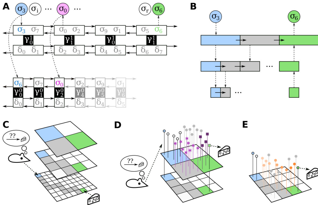
Figure 7: Retrieval of sequences with a scale-space in descending mode . (A) \gamma_i^{(n)} learn transitions in two spaces simultaneously (cf. Figure 3). During retrieval, one space is sufficient (dashed lines) and expansion starts on the highest level from start (blue circle) to goal (green circle). After an approximate solution was found on a level, sub-goals are generated (magenta circle). Then, the next lower scale computes expansions to these sub-goals. (B) Simplified depiction of (A) that omits details about the input spaces of transitions. (C) An animal wants to compute a path from its current location to a target using a Transition Scale-Space. (D) It can first compute an estimate on the highest scale, prune unnecessary symbols (gray circles), and generate sub-goals (magenta stars). (E) The trajectory is subsequently refined by planning on a finer scale to these sub-goals. Note that, in the discrete case, diagonal movements violate constant cost assumptions of MTS (see Waniek, 2018). In case of multiple viable trajectories, the algorithm chooses one arbitrarily.
