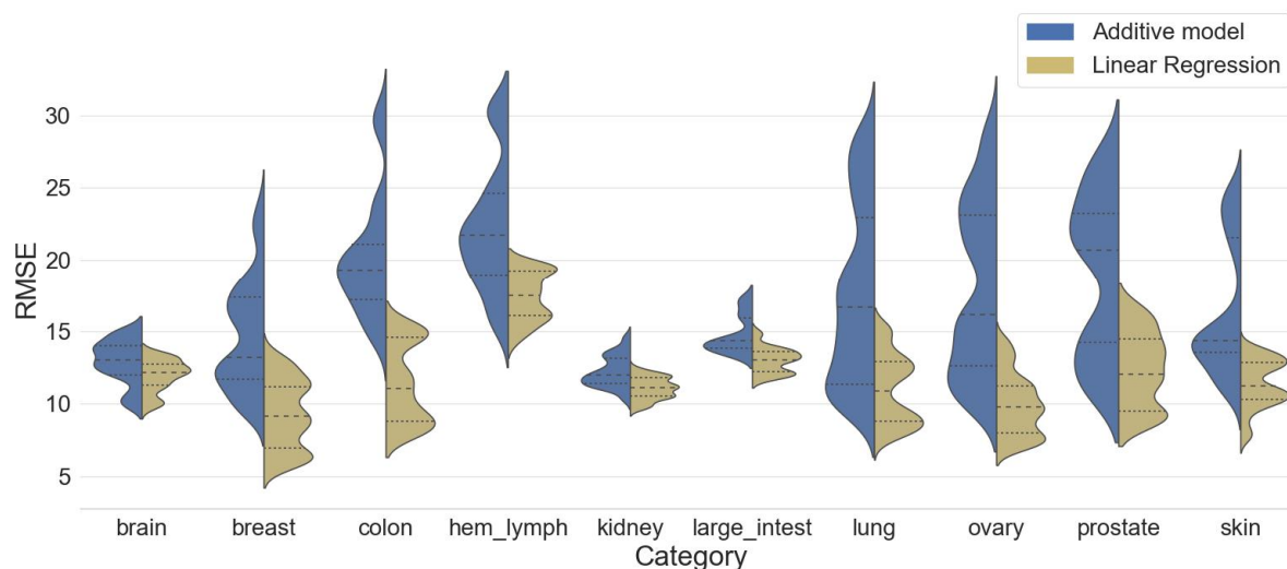
Figure 5. Performance of predicting CSS using linear regression as compared to the additive model. The RMSE for each cell line was grouped as density plots according to its tissue type. Dashed lines within each plot indicate interquartile range of the distribution.
