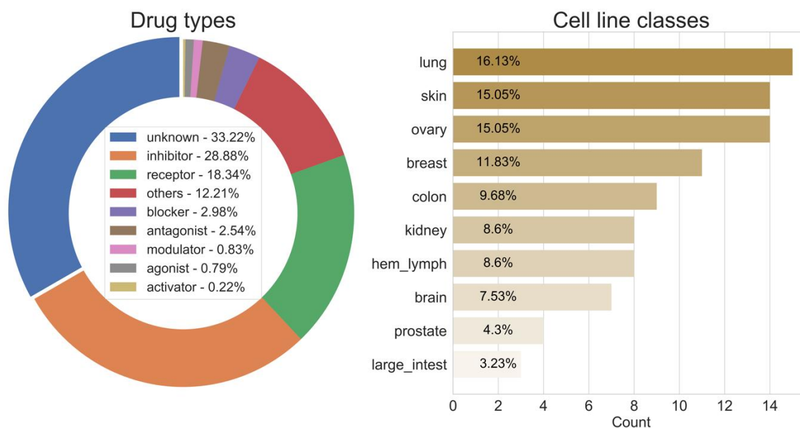
Figure 3. Classification of drugs and cell lines in DrugComb. Drugs were classified according to the mechanism types, following the ChEMBL implementation. Cell lines were classified according to the tissue of origin.
