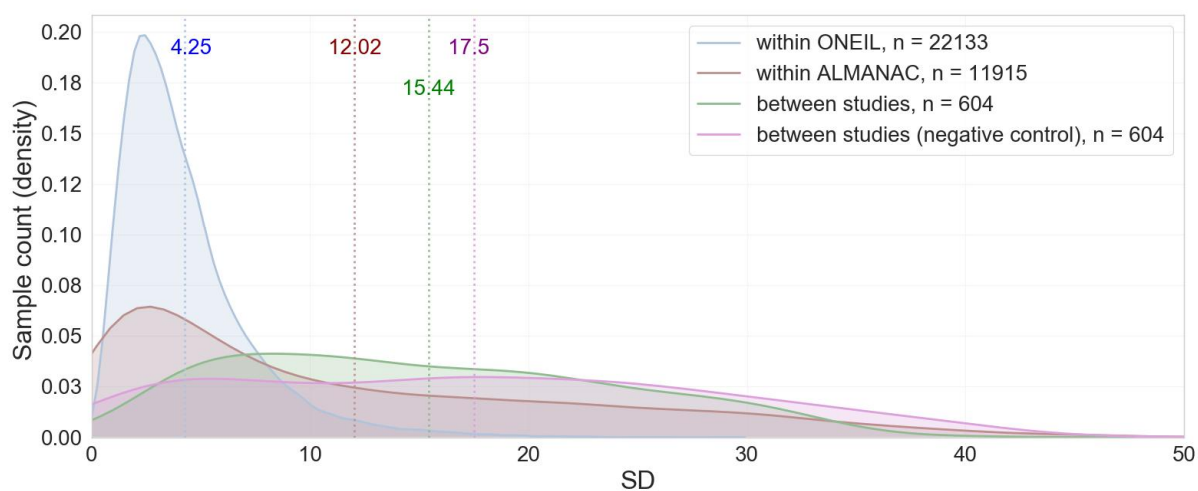
Figure 4. Replicability of drug combinations between and within studies represented as the distribution of the standard deviations of the Drug combination sensitivity scores (CSS). Mean values for each of the kernel density plots are delineated with a dotted line of corresponding color.
